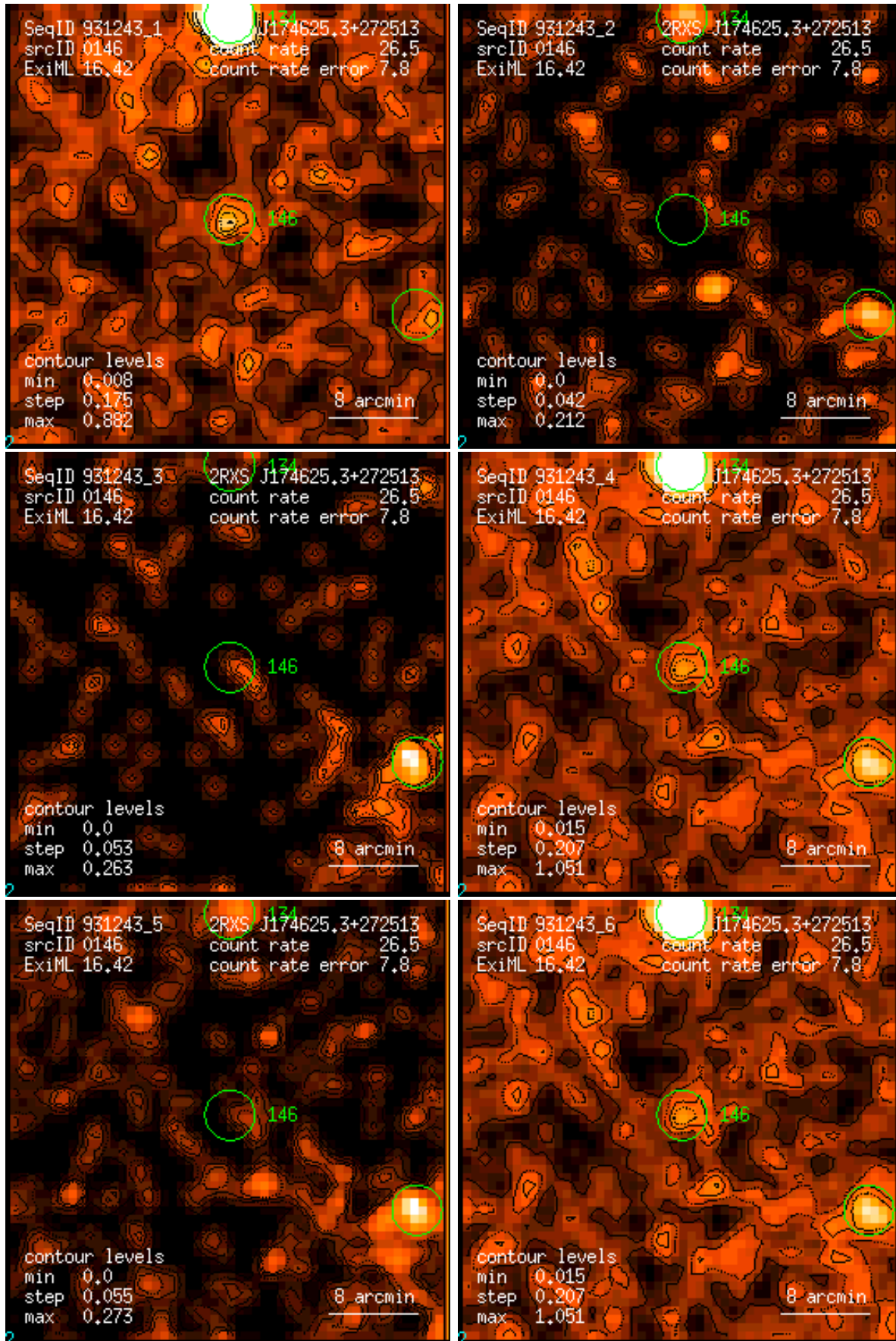
Figure 146: RASS 931243: detection 0146: band rate images, Gaussian filter: (1) PSPC channels 11 – 41, (2) 52 – 90, (3) 91 – 201, (4) 11 – 235, (5) 52 – 201, (6) 11 – 201. Broad band rates in counts/ks. Band rate contour levels in counts/ks/arcmin 2 .
