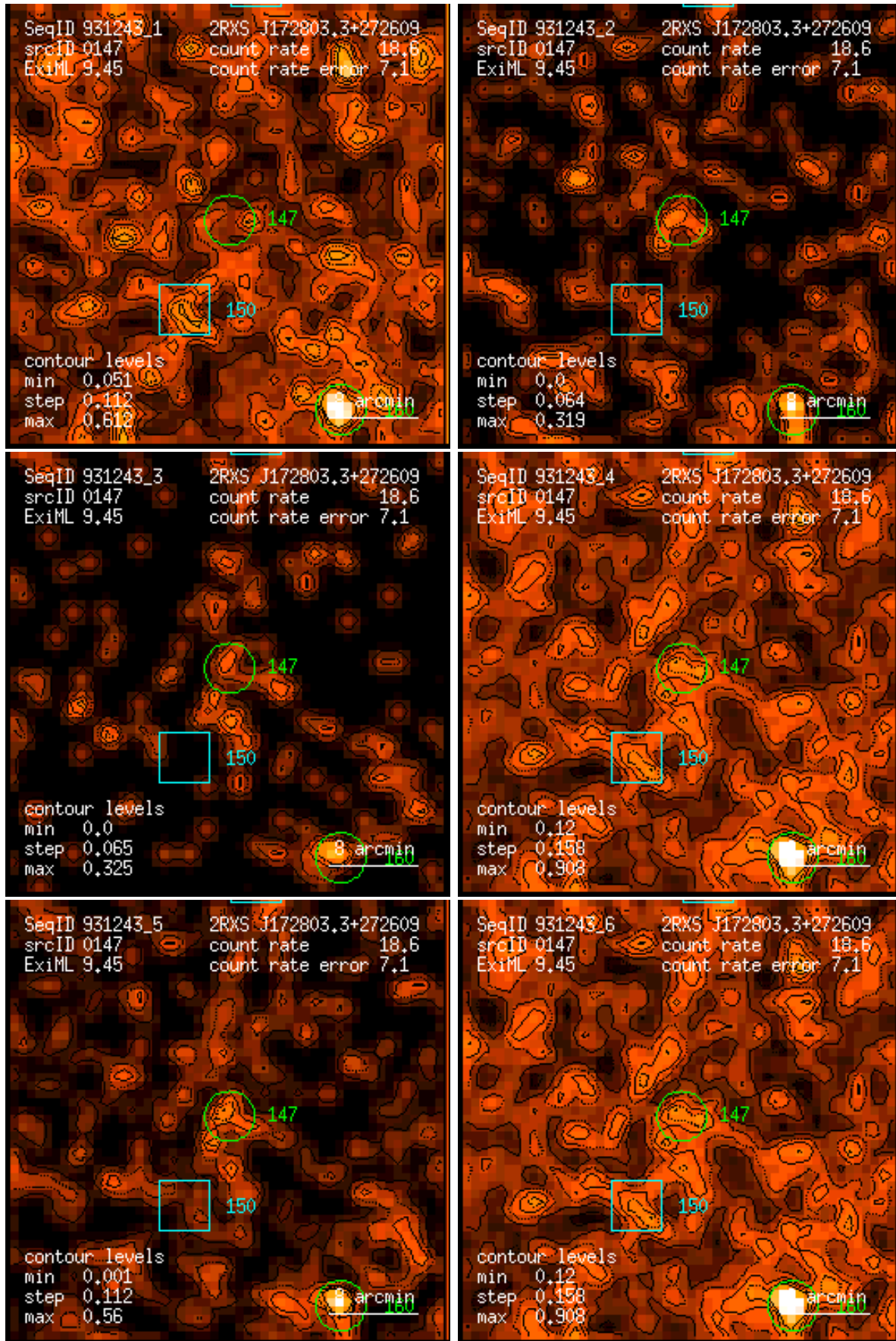
Figure 147: RASS 931243: detection 0147: band rate images, Gaussian filter: (1) PSPC channels 11 – 41, (2) 52 – 90, (3) 91 – 201, (4) 11 – 235, (5) 52 – 201, (6) 11 – 201. Broad band rates in counts/ks. Band rate contour levels in counts/ks/arcmin 2 .
