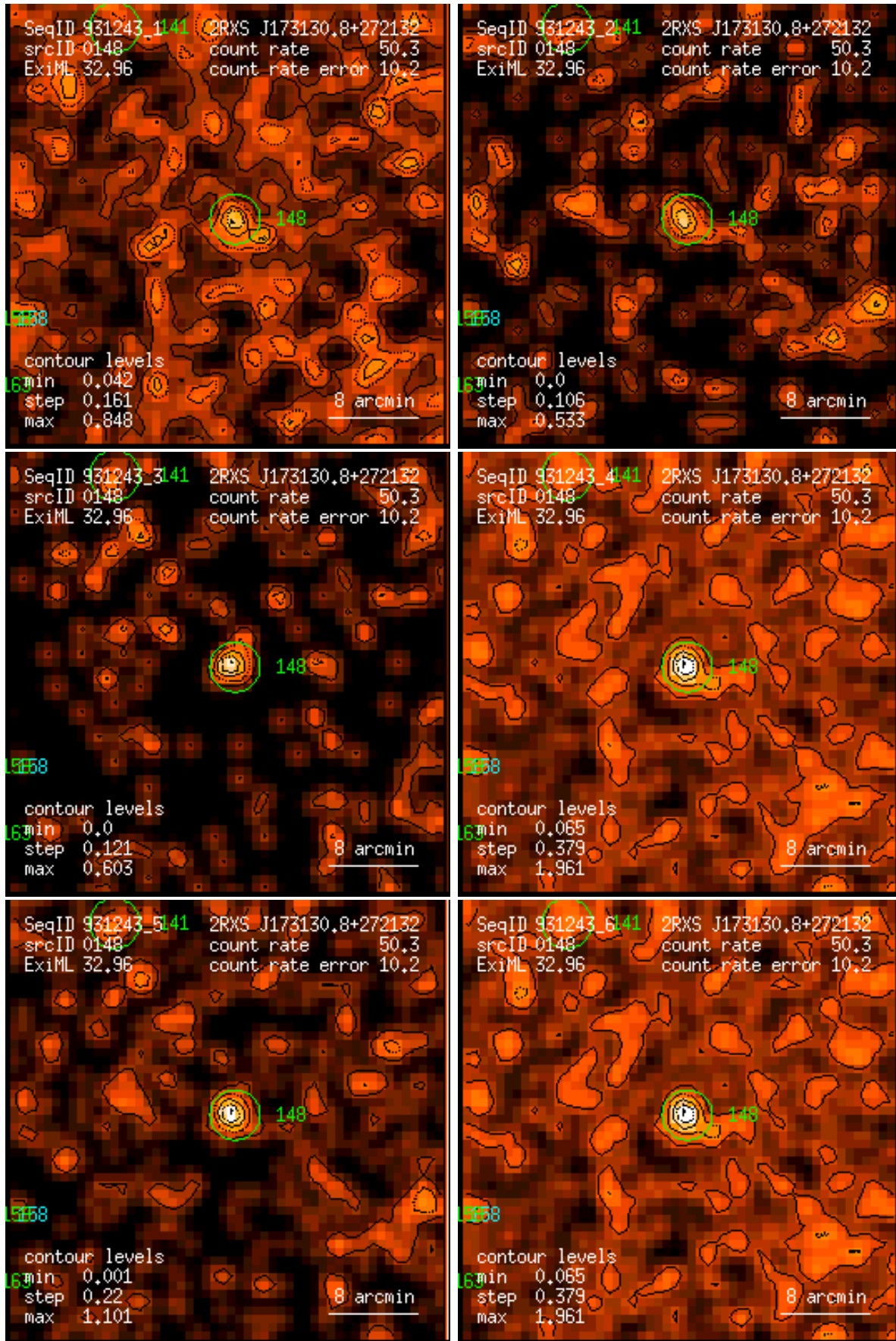
Figure 148: RASS 931243: detection 0148: band rate images, Gaussian filter: (1) PSPC channels 11 – 41, (2) 52 – 90, (3) 91 – 201, (4) 11 – 235, (5) 52 – 201, (6) 11 – 201. Broad band rates in counts/ks. Band rate contour levels in counts/ks/arcmin 2 .
