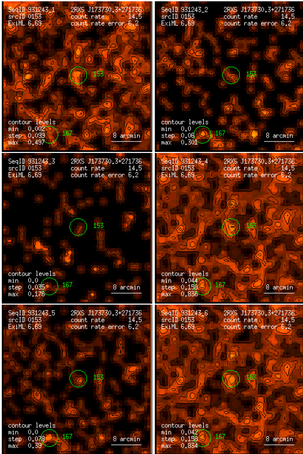
Figure 153: RASS 931243: detection 0153: band rate images, Gaussian filter: (1) PSPC channels 11 – 41, (2) 52 – 90, (3) 91 – 201, (4) 11 – 235, (5) 52 – 201, (6) 11 – 201. Broad band rates in counts/ks. Band rate contour levels in counts/ks/arcmin 2 .
