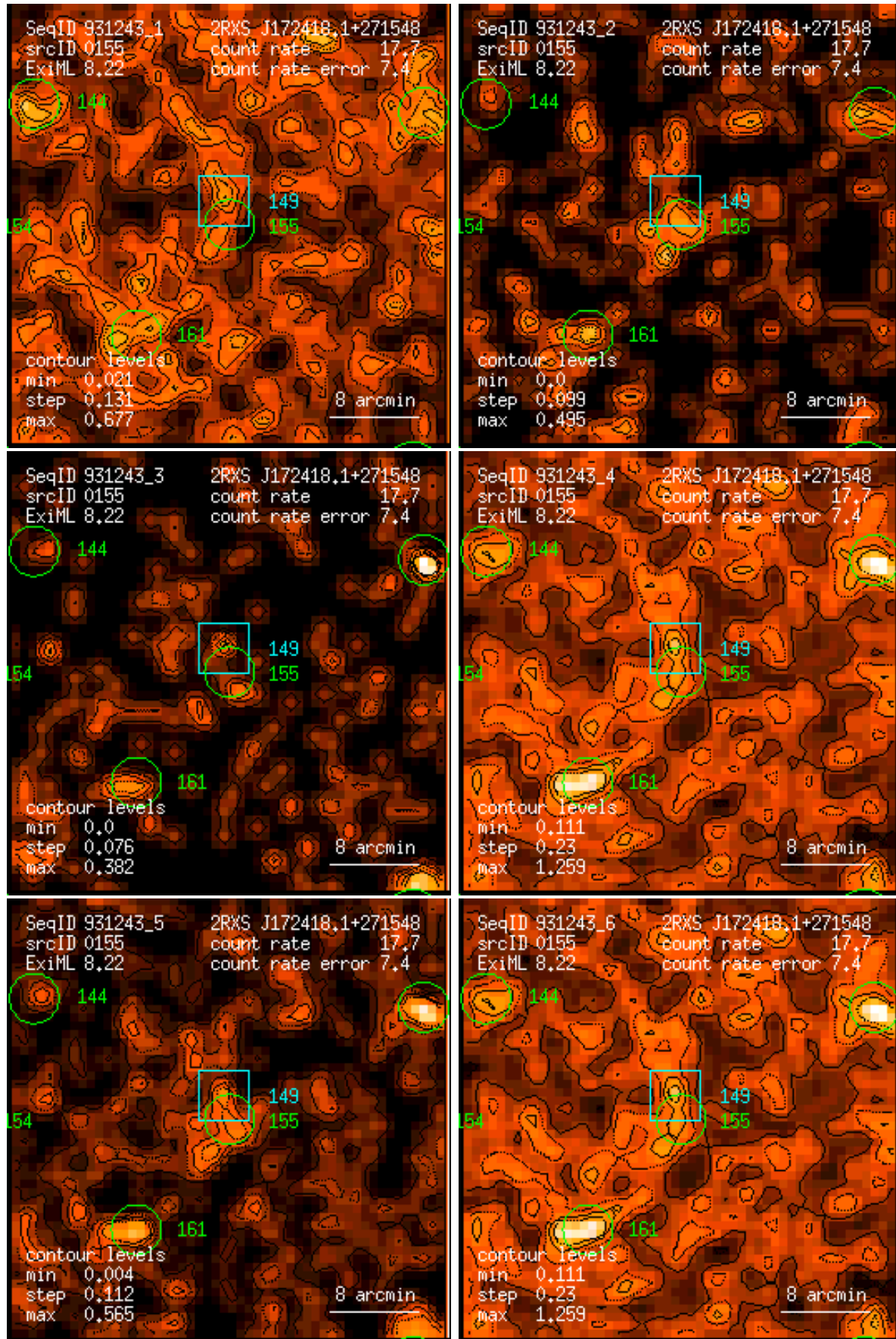
Figure 155: RASS 931243: detection 0155: band rate images, Gaussian filter: (1) PSPC channels 11 – 41, (2) 52 – 90, (3) 91 – 201, (4) 11 – 235, (5) 52 – 201, (6) 11 – 201. Broad band rates in counts/ks. Band rate contour levels in counts/ks/arcmin 2 .
