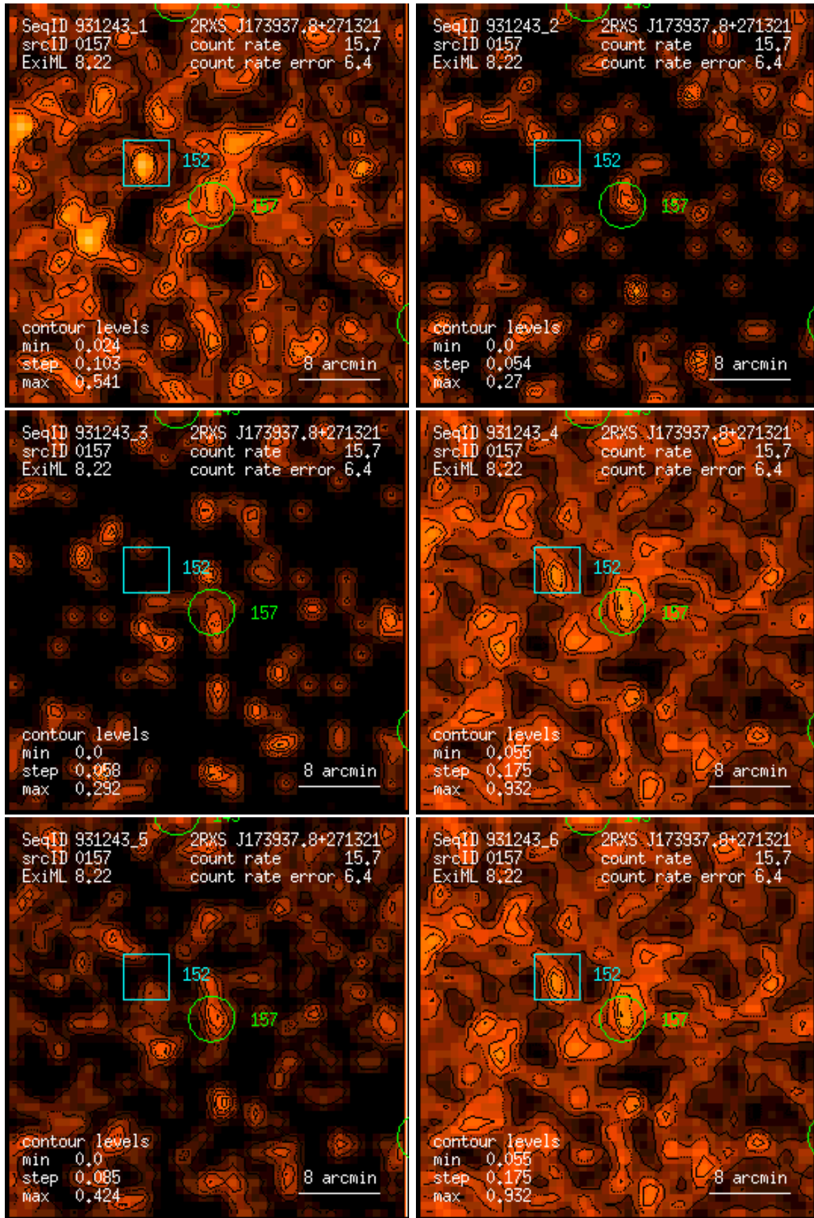
Figure 157: RASS 931243: detection 0157: band rate images, Gaussian filter: (1) PSPC channels 11 – 41, (2) 52 – 90, (3) 91 – 201, (4) 11 – 235, (5) 52 – 201, (6) 11 – 201. Broad band rates in counts/ks. Band rate contour levels in counts/ks/arcmin 2 .
