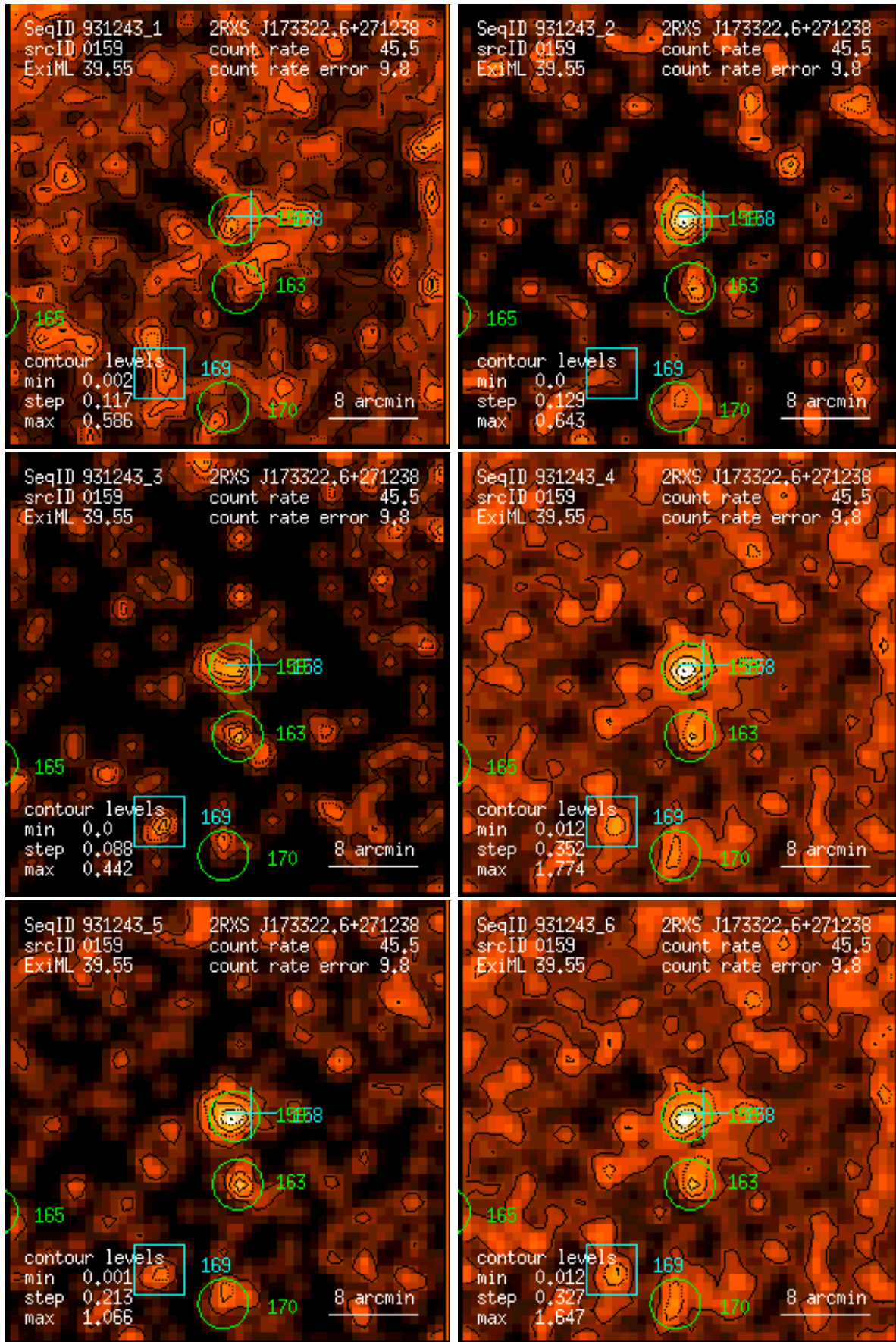
Figure 159: RASS 931243: detection 0159: band rate images, Gaussian filter: (1) PSPC channels 11 – 41, (2) 52 – 90, (3) 91 – 201, (4) 11 – 235, (5) 52 – 201, (6) 11 – 201. Broad band rates in counts/ks. Band rate contour levels in counts/ks/arcmin 2 .
