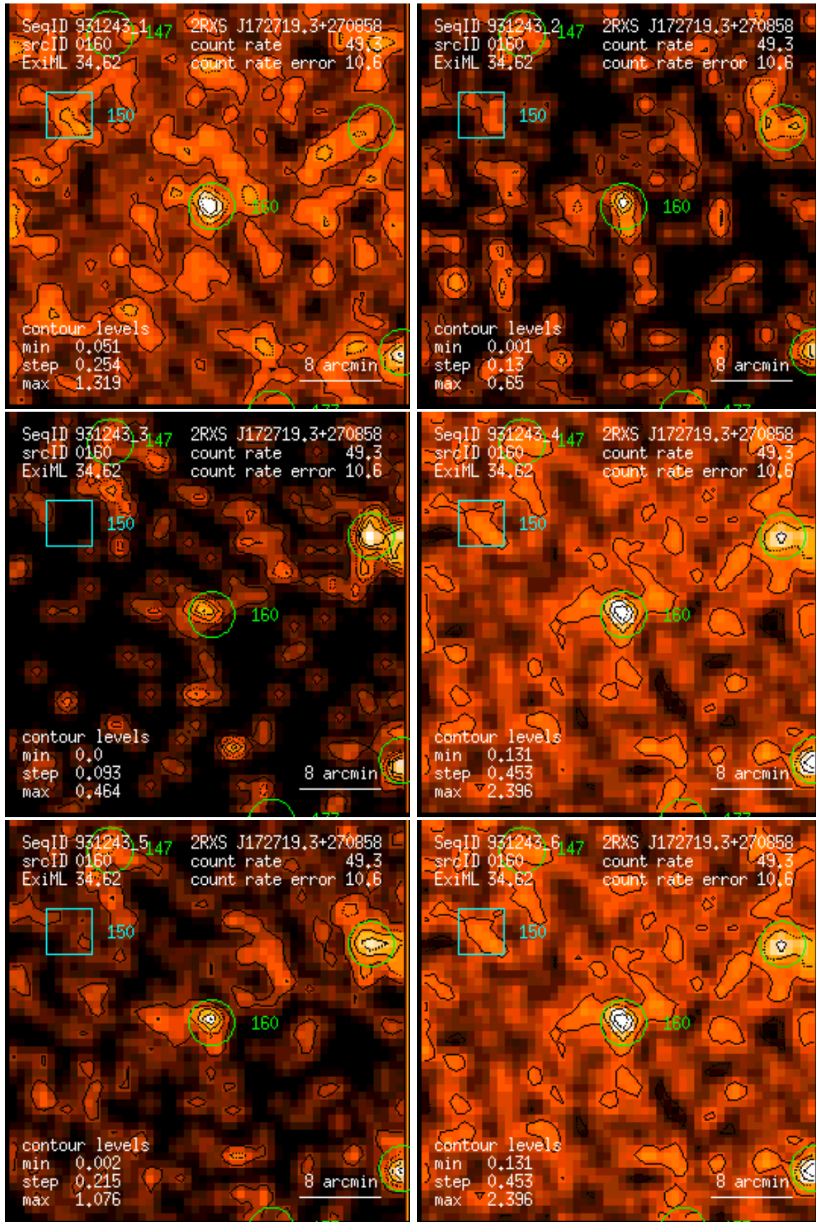
Figure 160: RASS 931243: detection 0160: band rate images, Gaussian filter: (1) PSPC channels 11 – 41, (2) 52 – 90, (3) 91 – 201, (4) 11 – 235, (5) 52 – 201, (6) 11 – 201. Broad band rates in counts/ks. Band rate contour levels in counts/ks/arcmin 2 .
