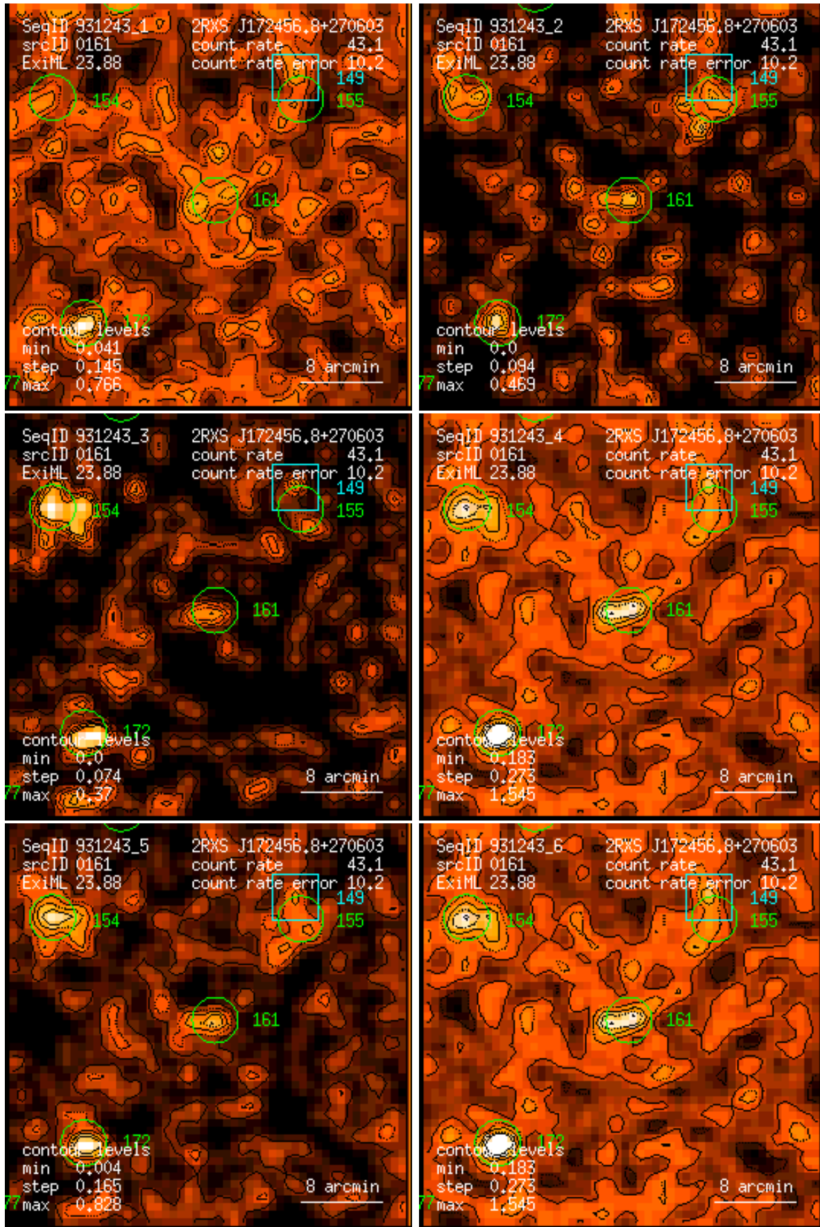
Figure 161: RASS 931243: detection 0161: band rate images, Gaussian filter: (1) PSPC channels 11 – 41, (2) 52 – 90, (3) 91 – 201, (4) 11 – 235, (5) 52 – 201, (6) 11 – 201. Broad band rates in counts/ks. Band rate contour levels in counts/ks/arcmin 2 .
