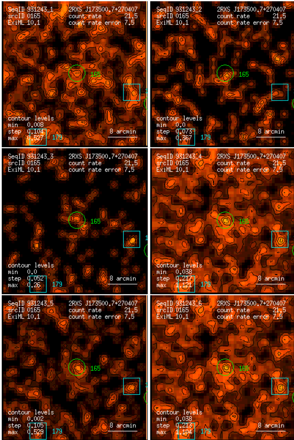
Figure 165: RASS 931243: detection 0165: band rate images, Gaussian filter: (1) PSPC channels 11 – 41, (2) 52 – 90, (3) 91 – 201, (4) 11 – 235, (5) 52 – 201, (6) 11 – 201. Broad band rates in counts/ks. Band rate contour levels in counts/ks/arcmin 2 .
