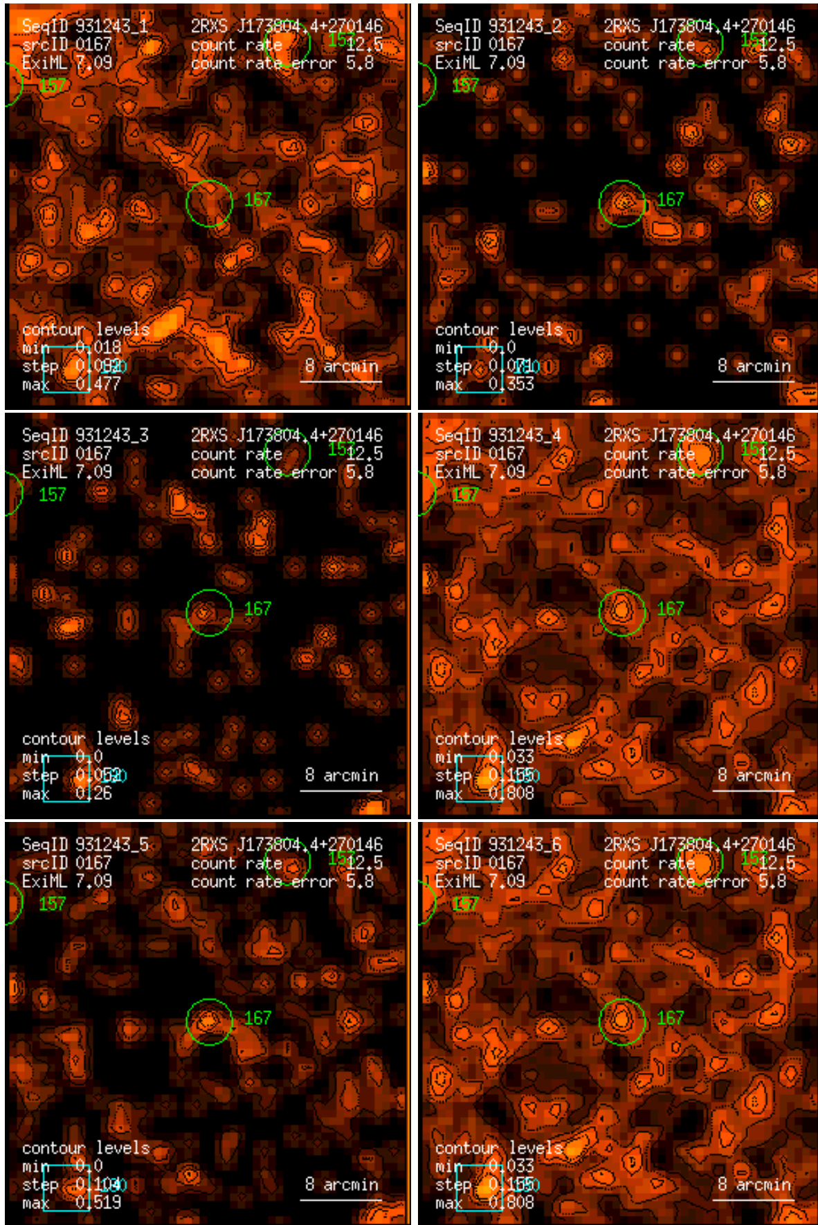
Figure 167: RASS 931243: detection 0167: band rate images, Gaussian filter: (1) PSPC channels 11 – 41, (2) 52 – 90, (3) 91 – 201, (4) 11 – 235, (5) 52 – 201, (6) 11 – 201. Broad band rates in counts/ks. Band rate contour levels in counts/ks/arcmin 2 .
