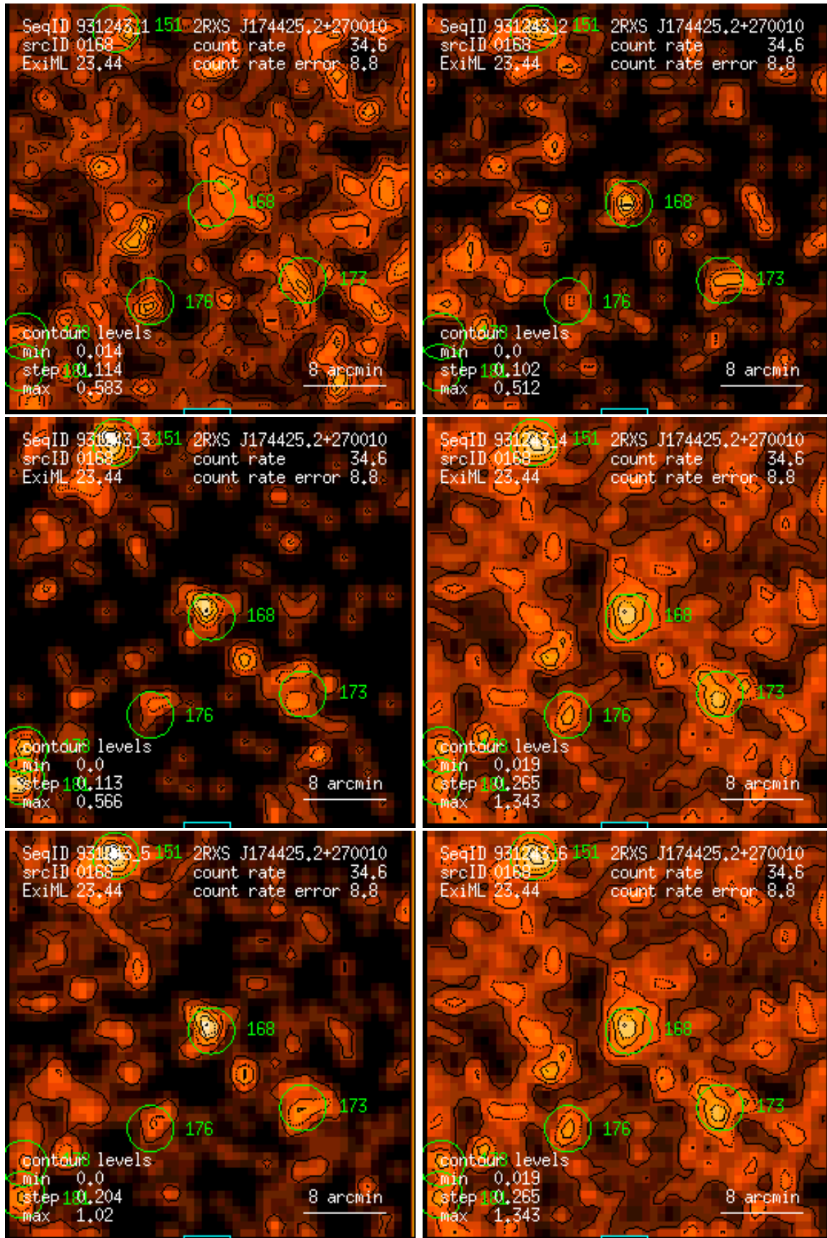
Figure 168: RASS 931243: detection 0168: band rate images, Gaussian filter: (1) PSPC channels 11 – 41, (2) 52 – 90, (3) 91 – 201, (4) 11 – 235, (5) 52 – 201, (6) 11 – 201. Broad band rates in counts/ks. Band rate contour levels in counts/ks/arcmin 2 .
