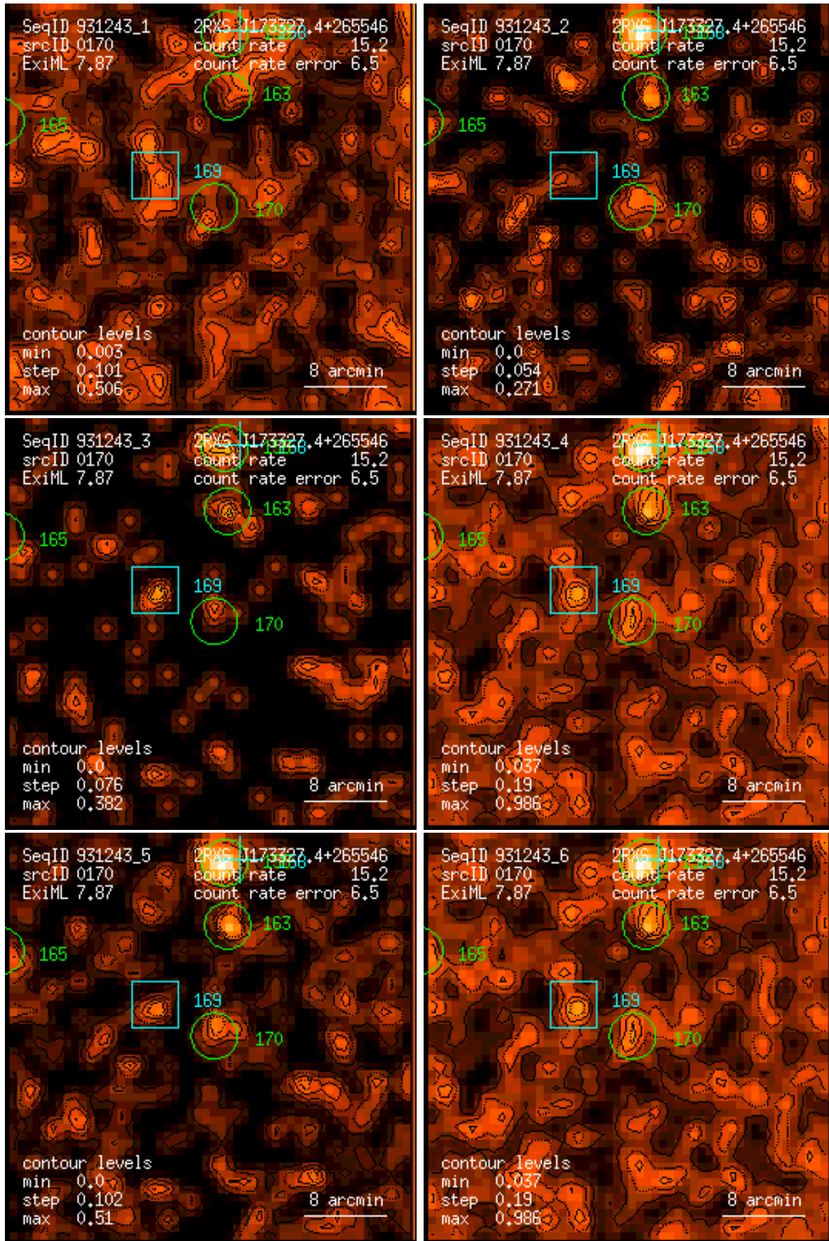
Figure 170: RASS 931243: detection 0170: band rate images, Gaussian filter: (1) PSPC channels 11 – 41, (2) 52 – 90, (3) 91 – 201, (4) 11 – 235, (5) 52 – 201, (6) 11 – 201. Broad band rates in counts/ks. Band rate contour levels in counts/ks/arcmin 2 .
