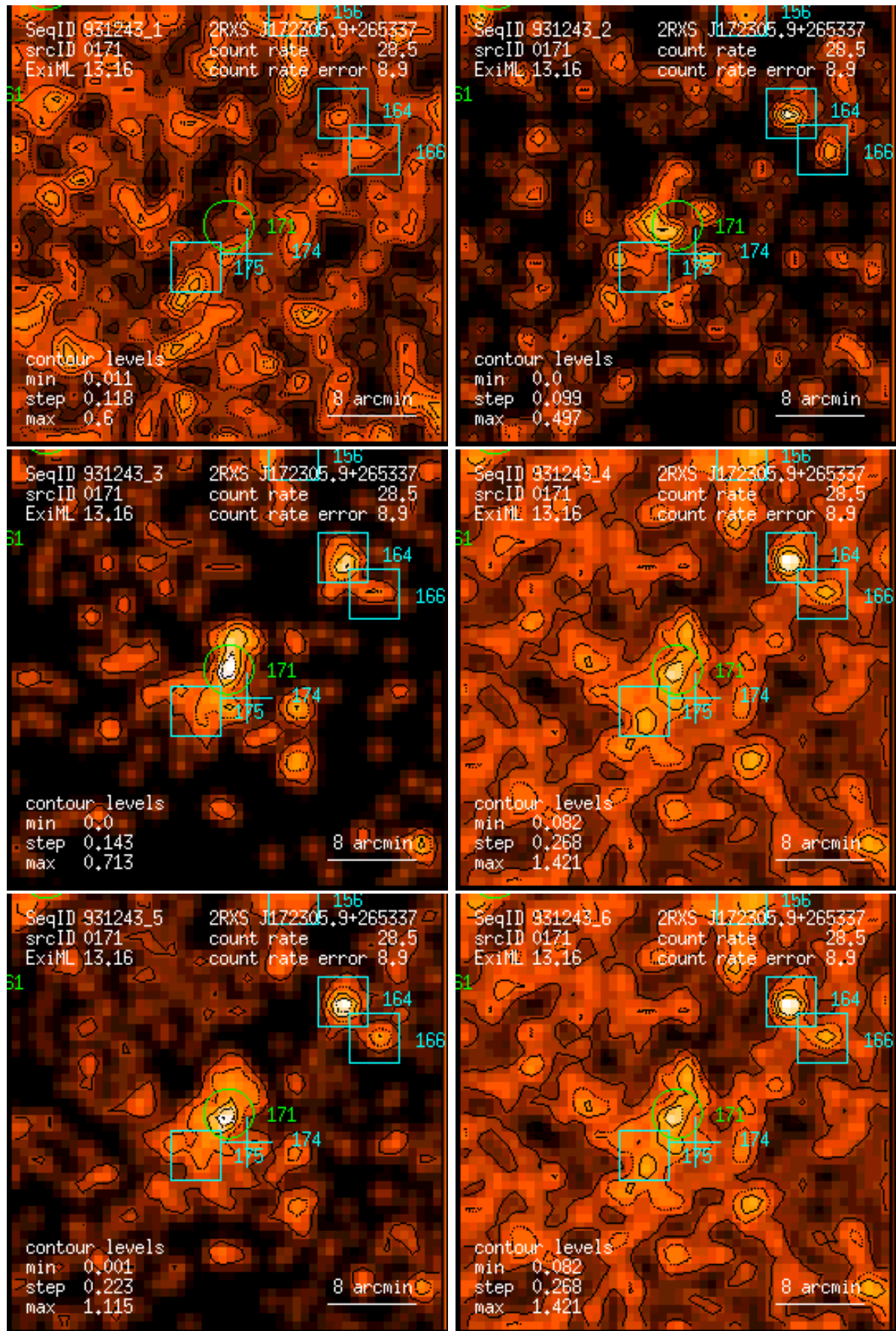
Figure 171: RASS 931243: detection 0171: band rate images, Gaussian filter: (1) PSPC channels 11 – 41, (2) 52 – 90, (3) 91 – 201, (4) 11 – 235, (5) 52 – 201, (6) 11 – 201. Broad band rates in counts/ks. Band rate contour levels in counts/ks/arcmin 2 .
