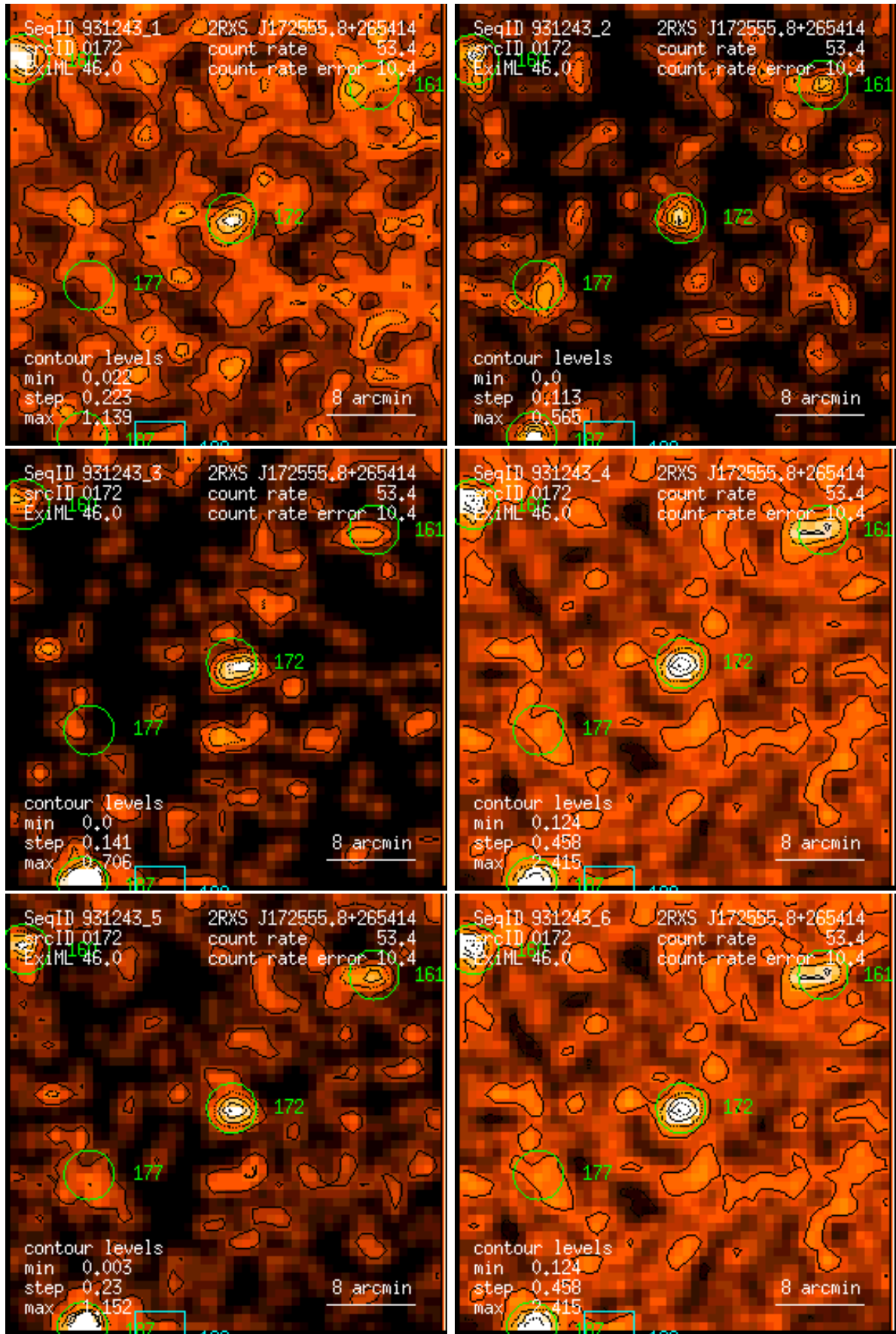
Figure 172: RASS 931243: detection 0172: band rate images, Gaussian filter: (1) PSPC channels 11 – 41, (2) 52 – 90, (3) 91 – 201, (4) 11 – 235, (5) 52 – 201, (6) 11 – 201. Broad band rates in counts/ks. Band rate contour levels in counts/ks/arcmin 2 .
