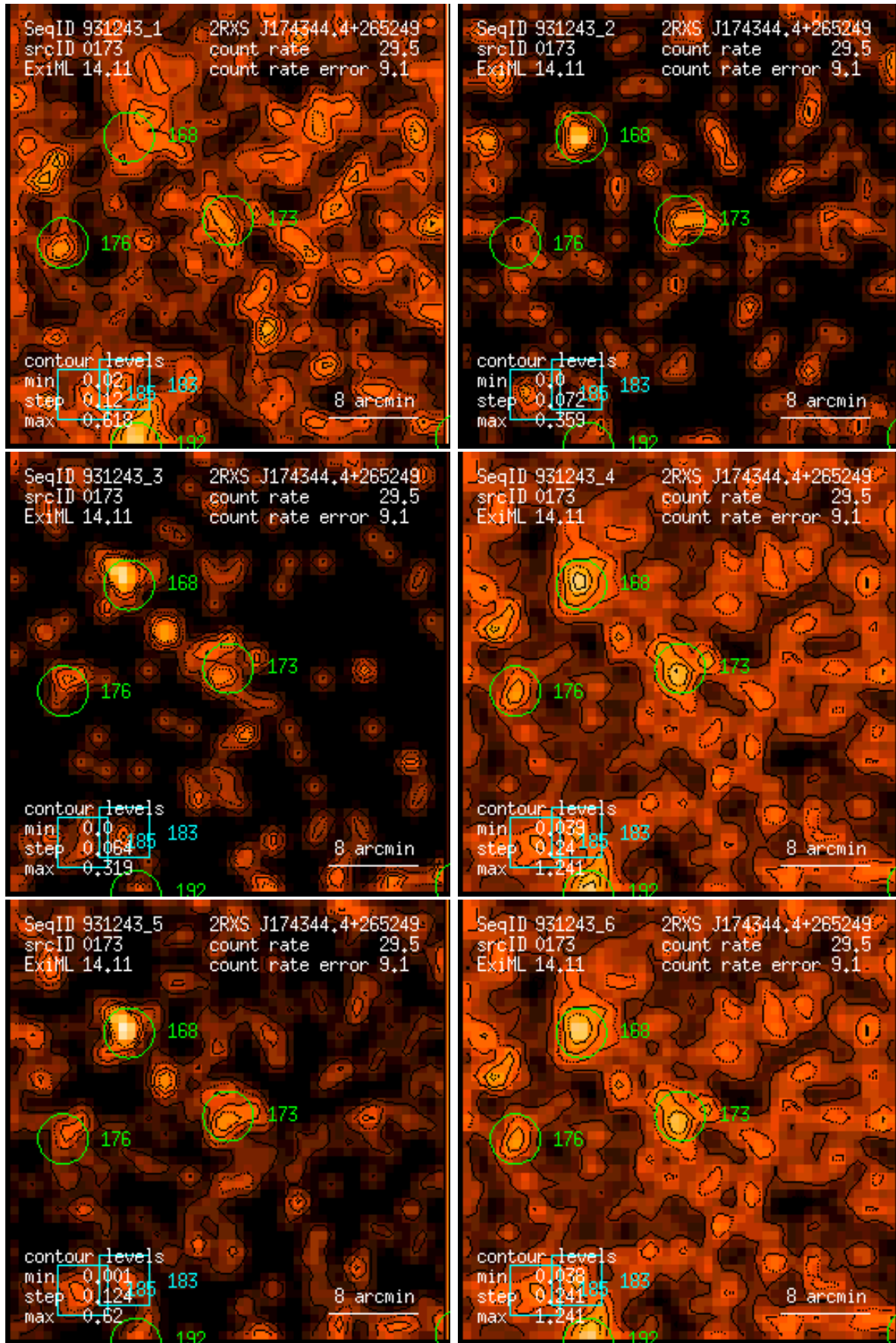
Figure 173: RASS 931243: detection 0173: band rate images, Gaussian filter: (1) PSPC channels 11 – 41, (2) 52 – 90, (3) 91 – 201, (4) 11 – 235, (5) 52 – 201, (6) 11 – 201. Broad band rates in counts/ks. Band rate contour levels in counts/ks/arcmin 2 .
