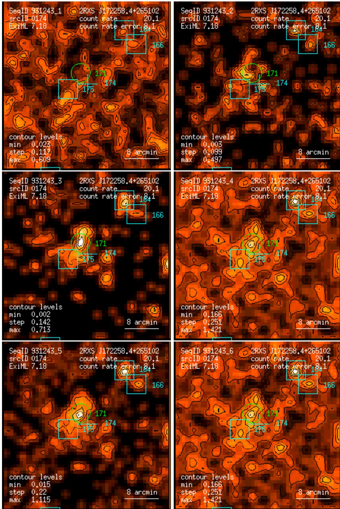
Figure 174: RASS 931243: detection 0174: band rate images, Gaussian filter: (1) PSPC channels 11 – 41, (2) 52 – 90, (3) 91 – 201, (4) 11 – 235, (5) 52 – 201, (6) 11 – 201. Broad band rates in counts/ks. Band rate contour levels in counts/ks/arcmin 2 .
