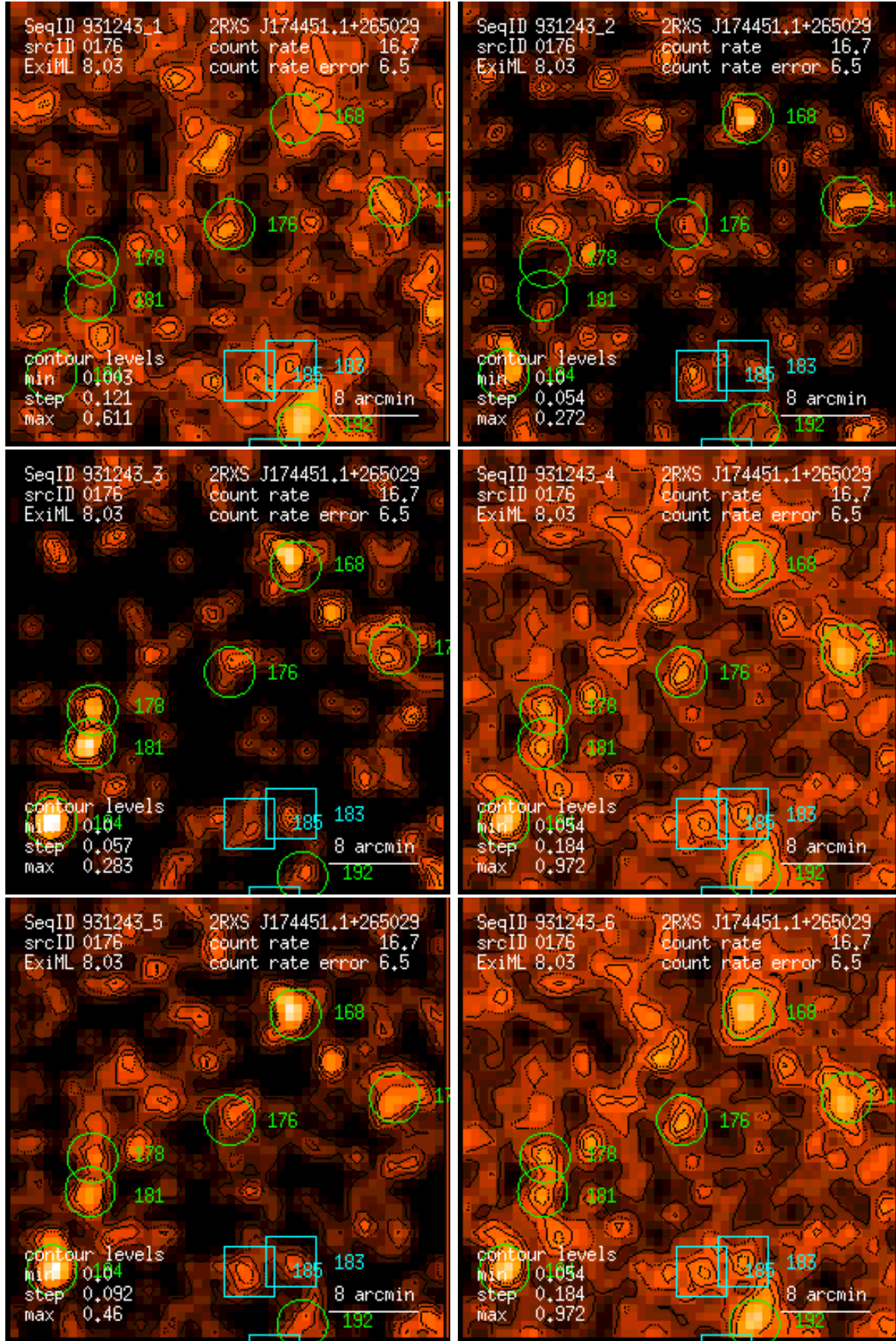
Figure 176: RASS 931243: detection 0176: band rate images, Gaussian filter: (1) PSPC channels 11 – 41, (2) 52 – 90, (3) 91 – 201, (4) 11 – 235, (5) 52 – 201, (6) 11 – 201. Broad band rates in counts/ks. Band rate contour levels in counts/ks/arcmin 2 .
