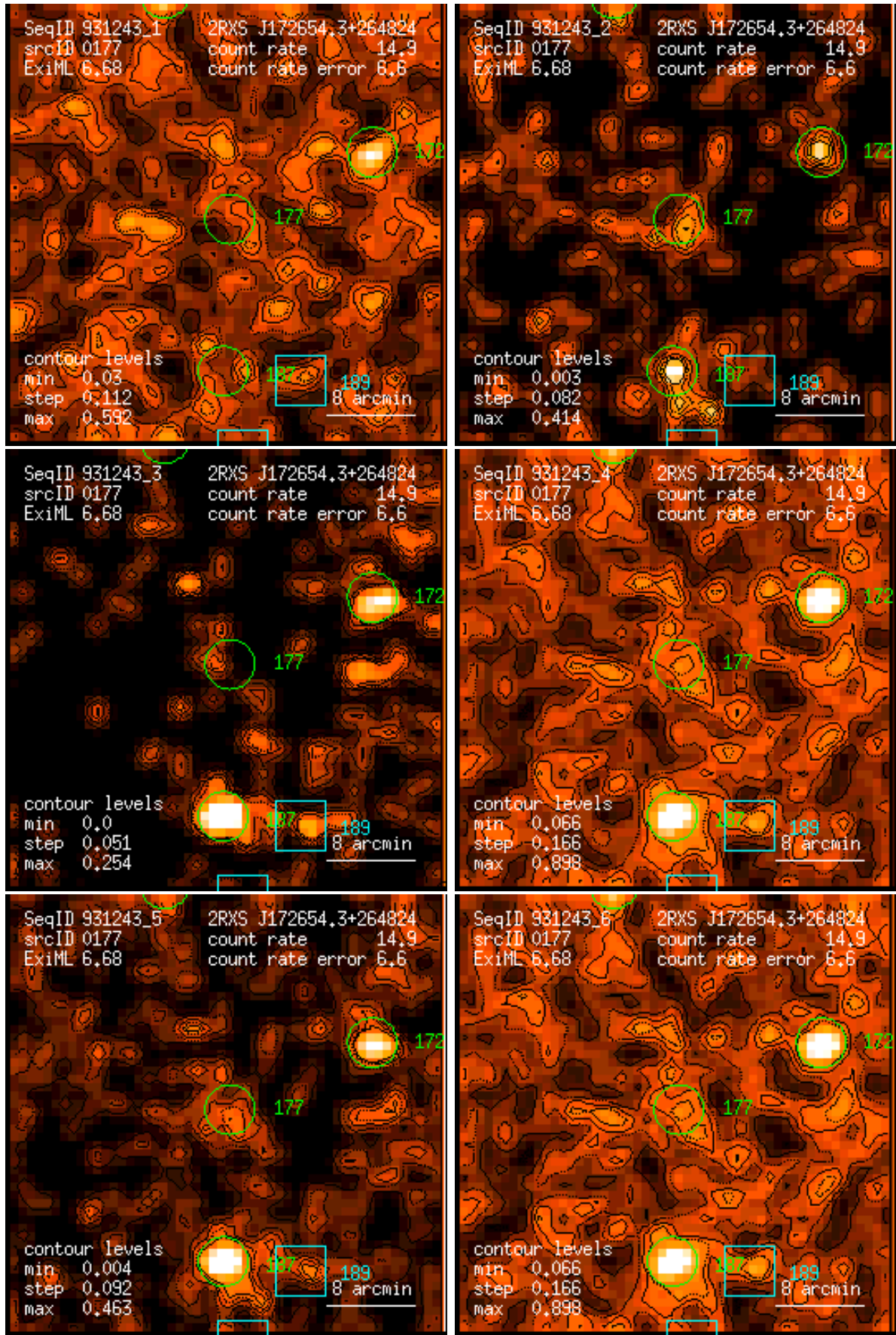
Figure 177: RASS 931243: detection 0177: band rate images, Gaussian filter: (1) PSPC channels 11 – 41, (2) 52 – 90, (3) 91 – 201, (4) 11 – 235, (5) 52 – 201, (6) 11 – 201. Broad band rates in counts/ks. Band rate contour levels in counts/ks/arcmin 2 .
