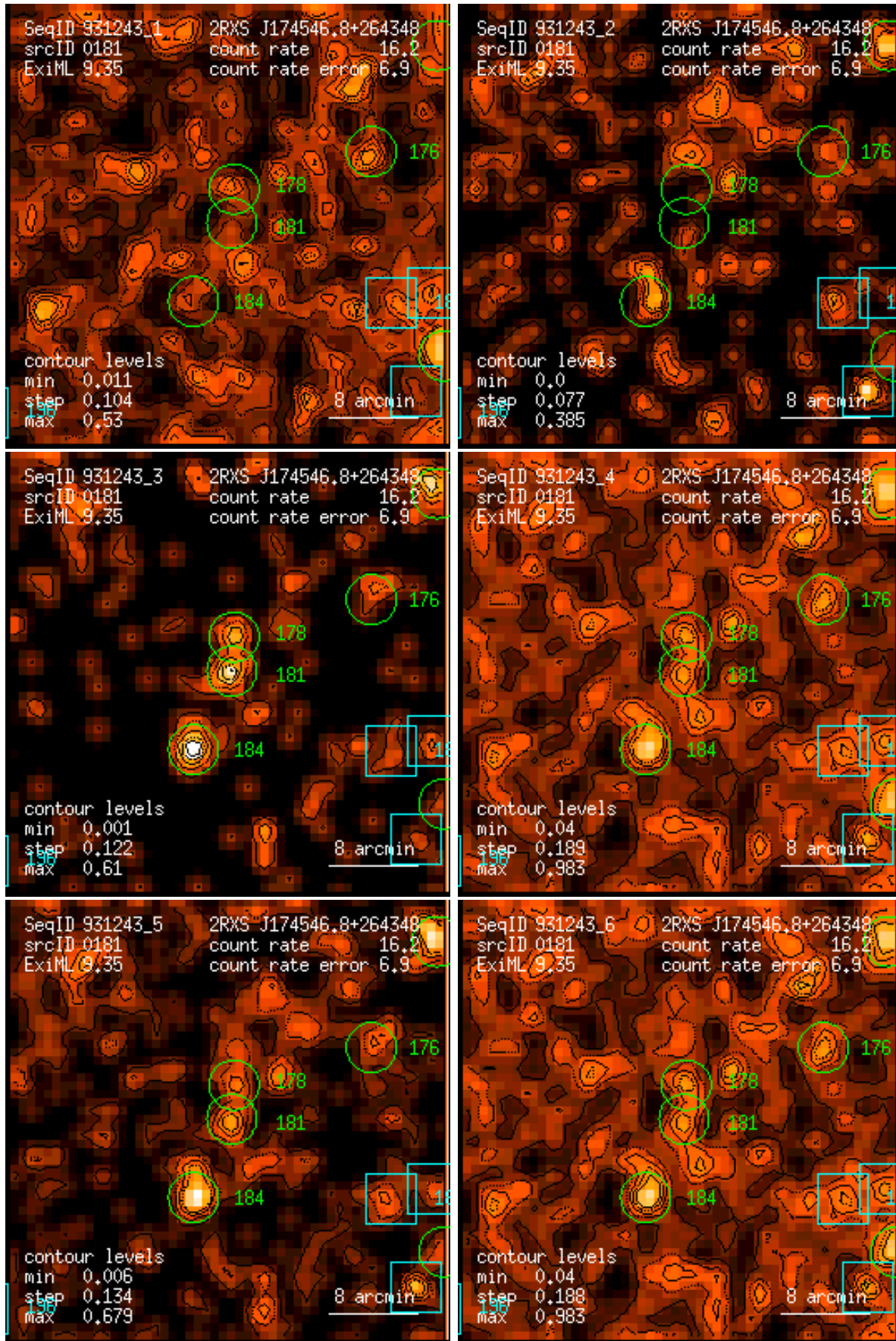
Figure 181: RASS 931243: detection 0181: band rate images, Gaussian filter: (1) PSPC channels 11 – 41, (2) 52 – 90, (3) 91 – 201, (4) 11 – 235, (5) 52 – 201, (6) 11 – 201. Broad band rates in counts/ks. Band rate contour levels in counts/ks/arcmin 2 .
