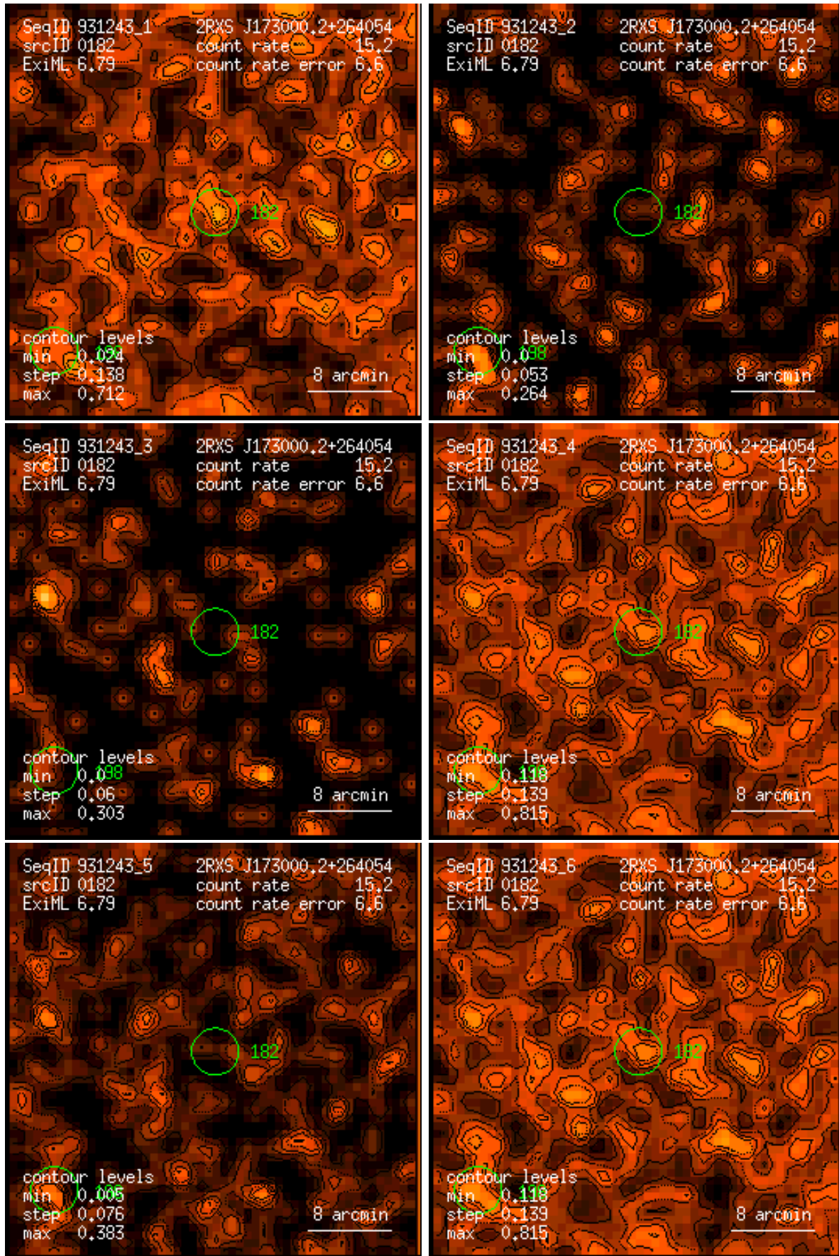
Figure 182: RASS 931243: detection 0182: band rate images, Gaussian filter: (1) PSPC channels 11 – 41, (2) 52 – 90, (3) 91 – 201, (4) 11 – 235, (5) 52 – 201, (6) 11 – 201. Broad band rates in counts/ks. Band rate contour levels in counts/ks/arcmin 2 .
