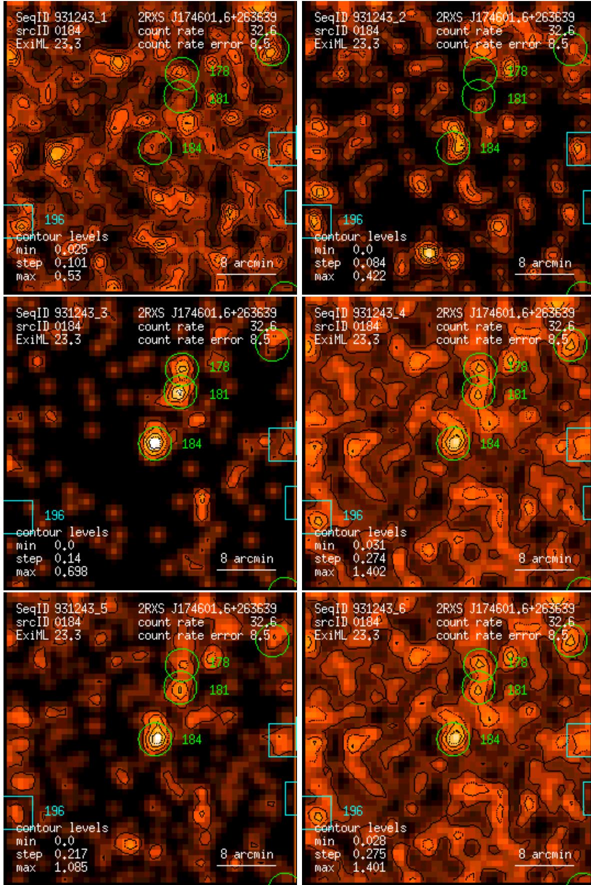
Figure 184: RASS 931243: detection 0184: band rate images, Gaussian filter: (1) PSPC channels 11 – 41, (2) 52 – 90, (3) 91 – 201, (4) 11 – 235, (5) 52 – 201, (6) 11 – 201. Broad band rates in counts/ks. Band rate contour levels in counts/ks/arcmin 2 .
