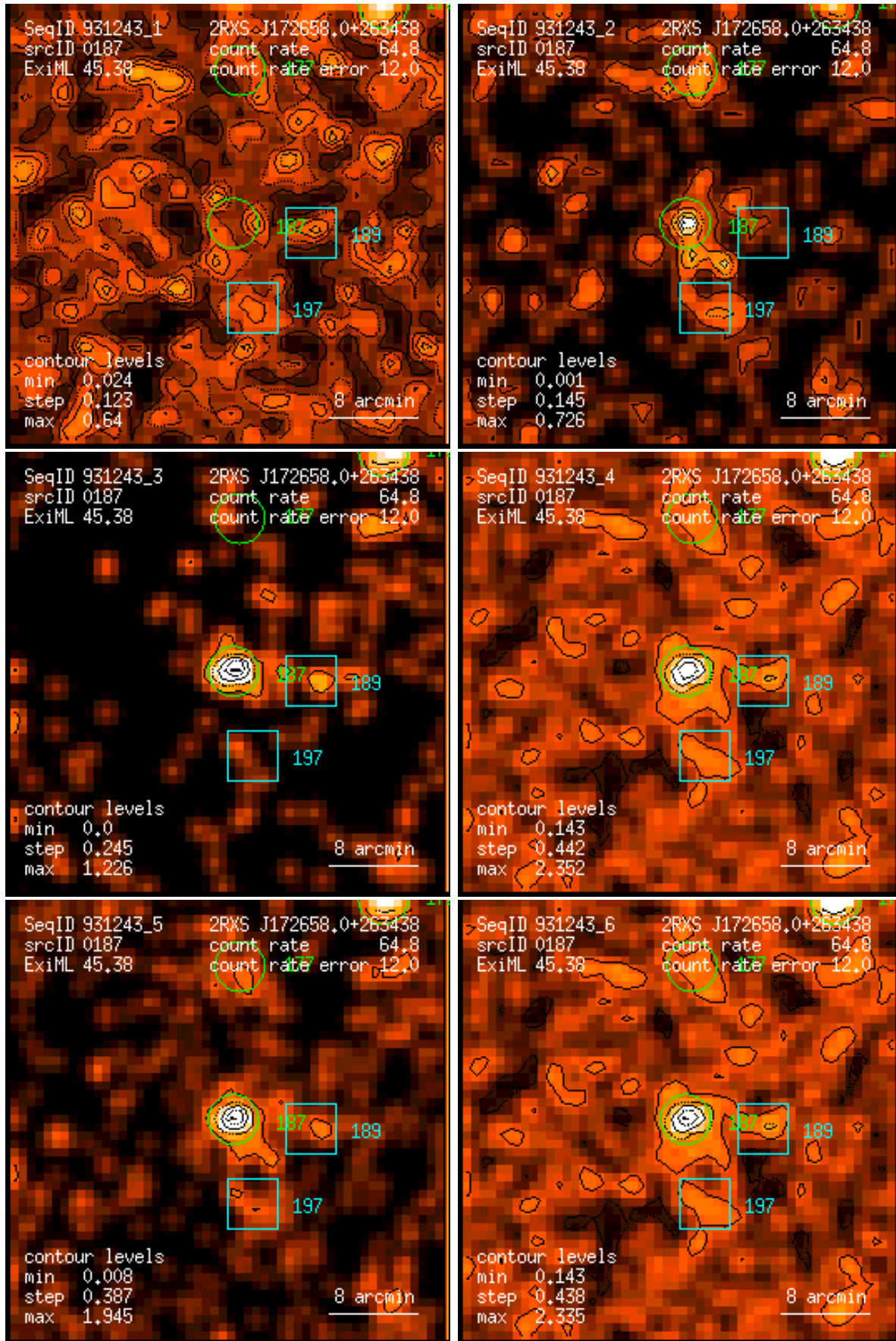
Figure 187: RASS 931243: detection 0187: band rate images, Gaussian filter: (1) PSPC channels 11 – 41, (2) 52 – 90, (3) 91 – 201, (4) 11 – 235, (5) 52 – 201, (6) 11 – 201. Broad band rates in counts/ks. Band rate contour levels in counts/ks/arcmin 2 .
