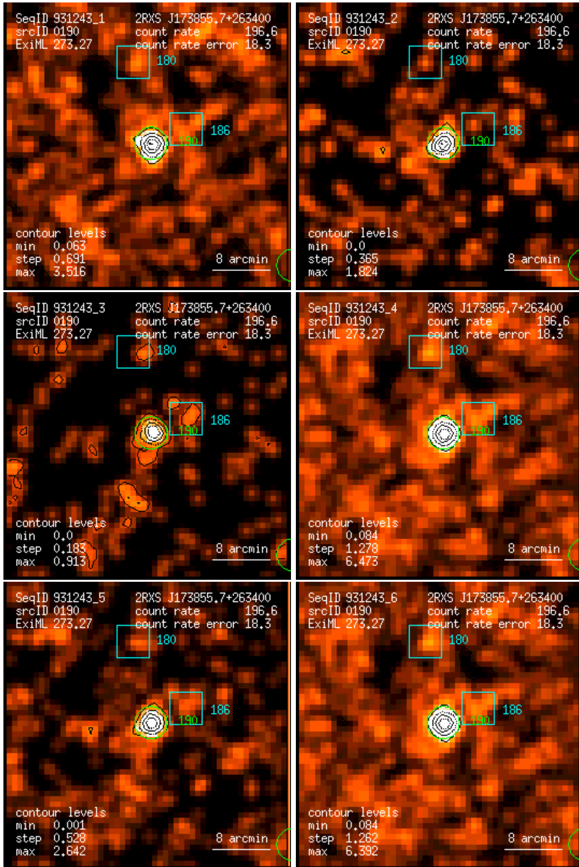
Figure 190: RASS 931243: detection 0190: band rate images, Gaussian filter: (1) PSPC channels 11 – 41, (2) 52 – 90, (3) 91 – 201, (4) 11 – 235, (5) 52 – 201, (6) 11 – 201. Broad band rates in counts/ks. Band rate contour levels in counts/ks/arcmin 2 .
