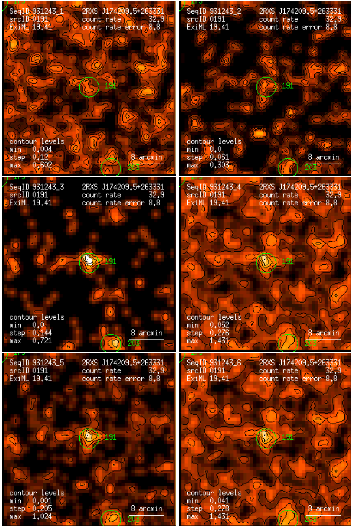
Figure 191: RASS 931243: detection 0191: band rate images, Gaussian filter: (1) PSPC channels 11 – 41, (2) 52 – 90, (3) 91 – 201, (4) 11 – 235, (5) 52 – 201, (6) 11 – 201. Broad band rates in counts/ks. Band rate contour levels in counts/ks/arcmin 2 .
