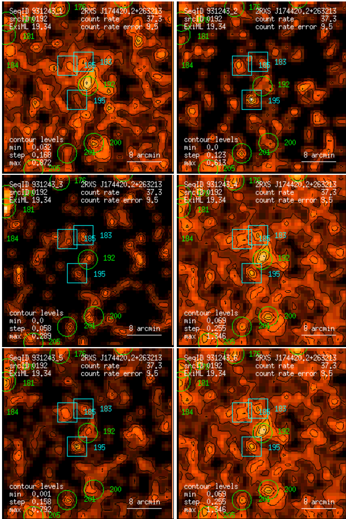
Figure 192: RASS 931243: detection 0192: band rate images, Gaussian filter: (1) PSPC channels 11 – 41, (2) 52 – 90, (3) 91 – 201, (4) 11 – 235, (5) 52 – 201, (6) 11 – 201. Broad band rates in counts/ks. Band rate contour levels in counts/ks/arcmin 2 .
