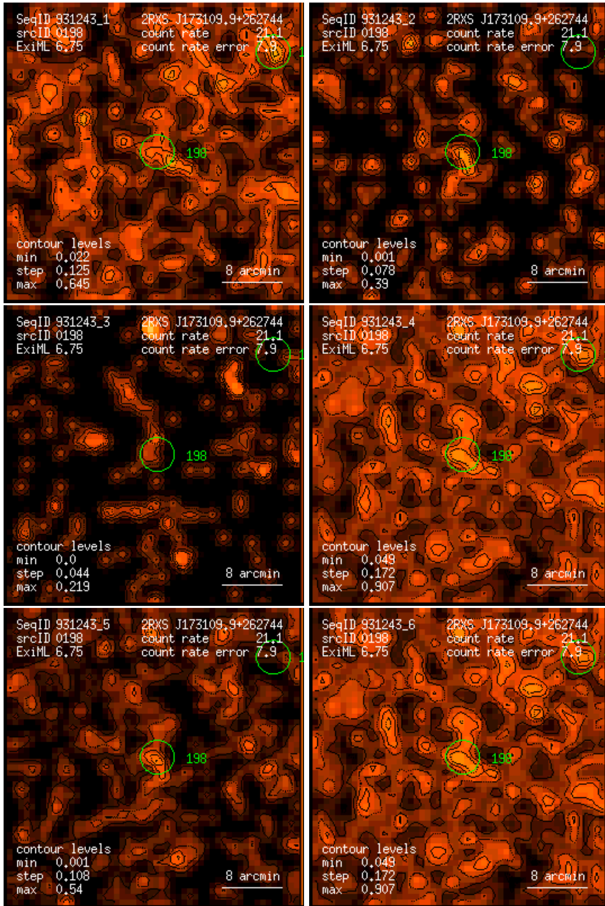
Figure 198: RASS 931243: detection 0198: band rate images, Gaussian filter: (1) PSPC channels 11 – 41, (2) 52 – 90, (3) 91 – 201, (4) 11 – 235, (5) 52 – 201, (6) 11 – 201. Broad band rates in counts/ks. Band rate contour levels in counts/ks/arcmin 2 .
