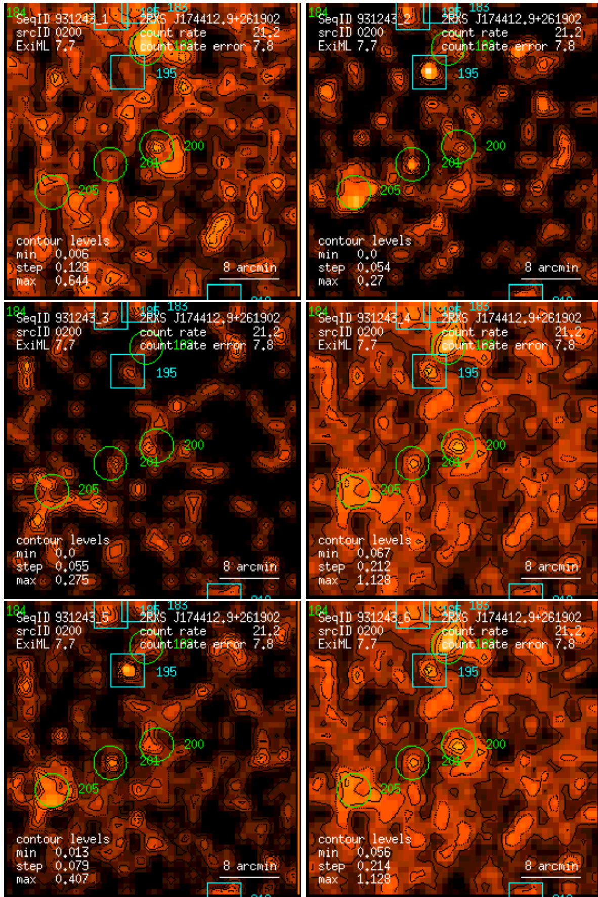
Figure 200: RASS 931243: detection 0200: band rate images, Gaussian filter: (1) PSPC channels 11 – 41, (2) 52 – 90, (3) 91 – 201, (4) 11 – 235, (5) 52 – 201, (6) 11 – 201. Broad band rates in counts/ks. Band rate contour levels in counts/ks/arcmin 2 .
