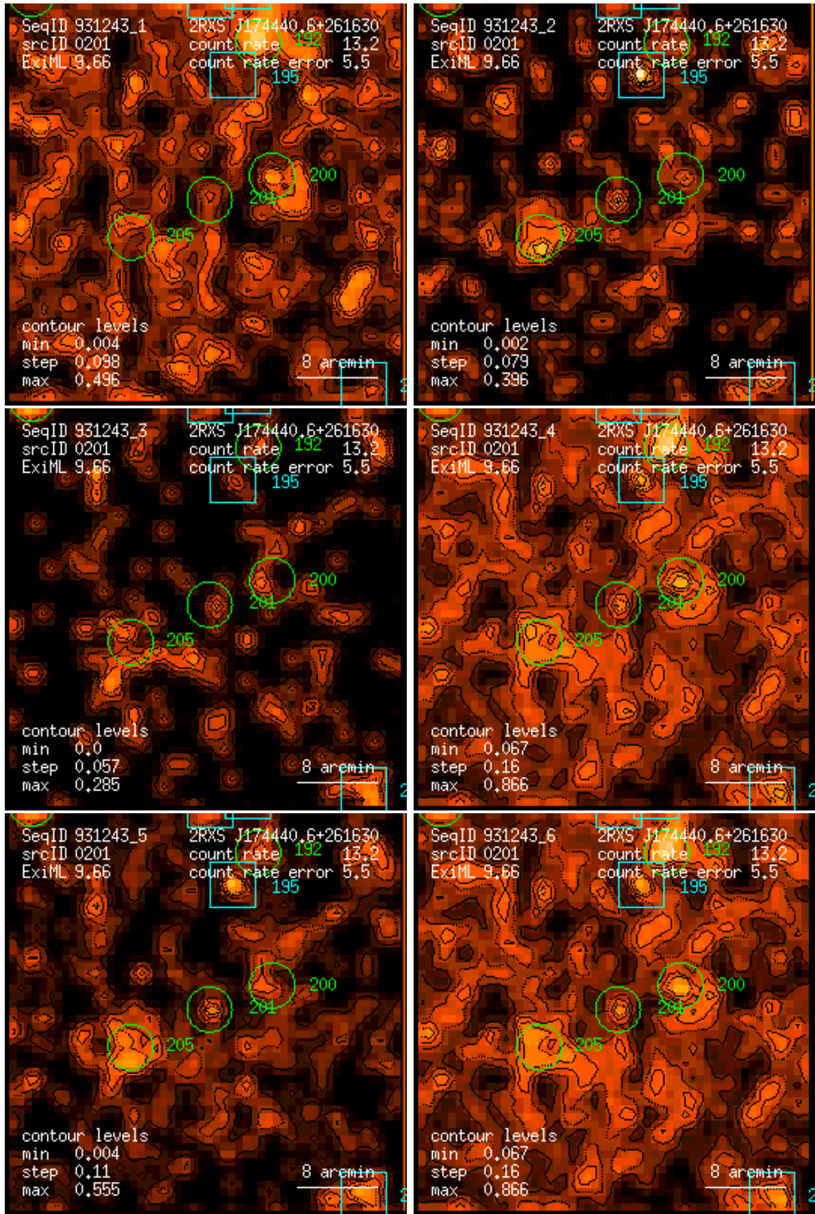
Figure 201: RASS 931243: detection 0201: band rate images, Gaussian filter: (1) PSPC channels 11 – 41, (2) 52 – 90, (3) 91 – 201, (4) 11 – 235, (5) 52 – 201, (6) 11 – 201. Broad band rates in counts/ks. Band rate contour levels in counts/ks/arcmin 2 .
