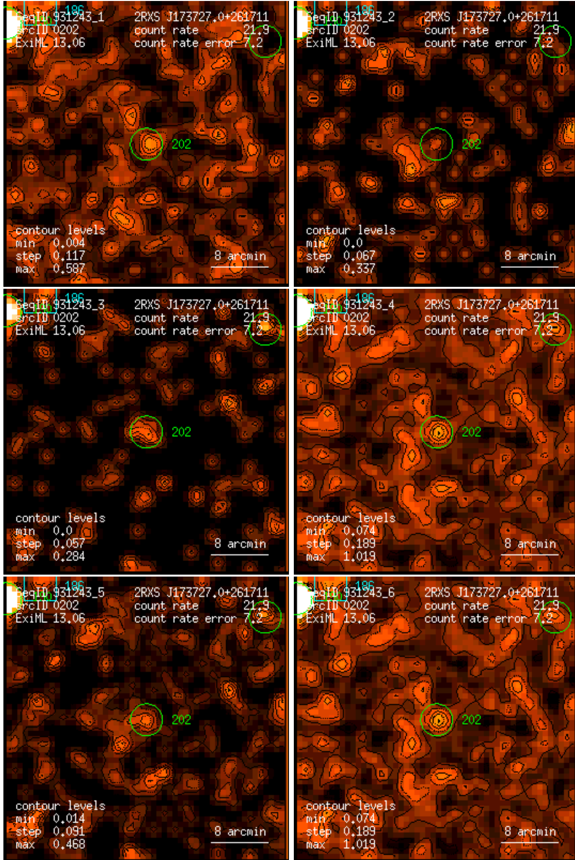
Figure 202: RASS 931243: detection 0202: band rate images, Gaussian filter: (1) PSPC channels 11 – 41, (2) 52 – 90, (3) 91 – 201, (4) 11 – 235, (5) 52 – 201, (6) 11 – 201. Broad band rates in counts/ks. Band rate contour levels in counts/ks/arcmin 2 .
