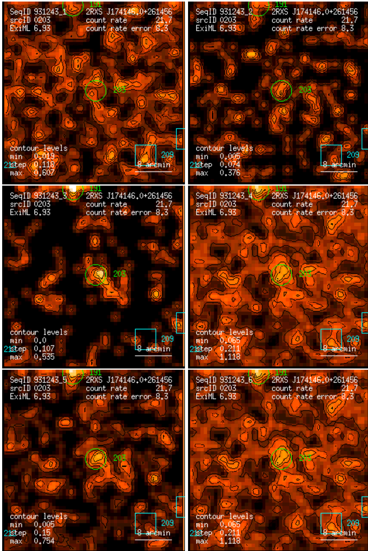
Figure 203: RASS 931243: detection 0203: band rate images, Gaussian filter: (1) PSPC channels 11 – 41, (2) 52 – 90, (3) 91 – 201, (4) 11 – 235, (5) 52 – 201, (6) 11 – 201. Broad band rates in counts/ks. Band rate contour levels in counts/ks/arcmin 2 .
