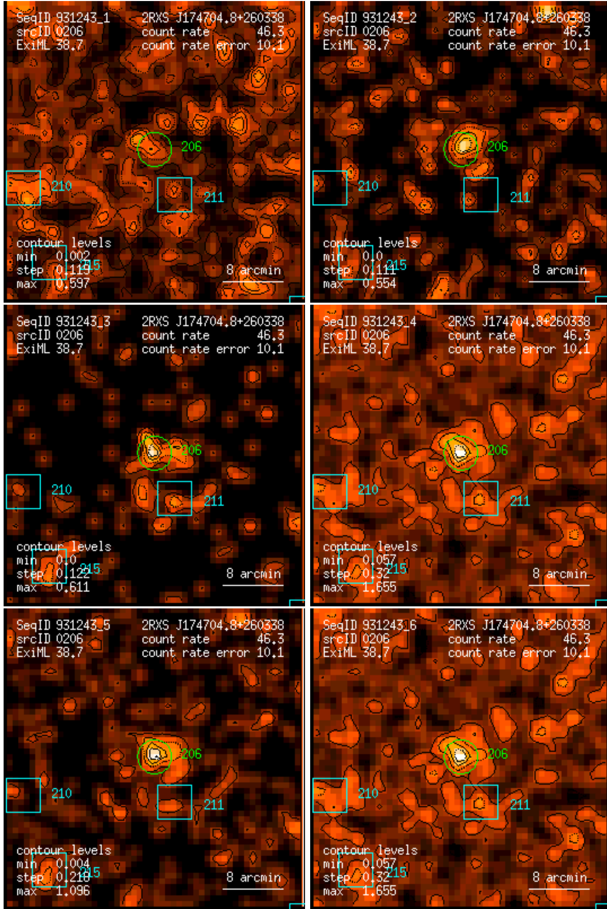
Figure 206: RASS 931243: detection 0206: band rate images, Gaussian filter: (1) PSPC channels 11 – 41, (2) 52 – 90, (3) 91 – 201, (4) 11 – 235, (5) 52 – 201, (6) 11 – 201. Broad band rates in counts/ks. Band rate contour levels in counts/ks/arcmin 2 .
