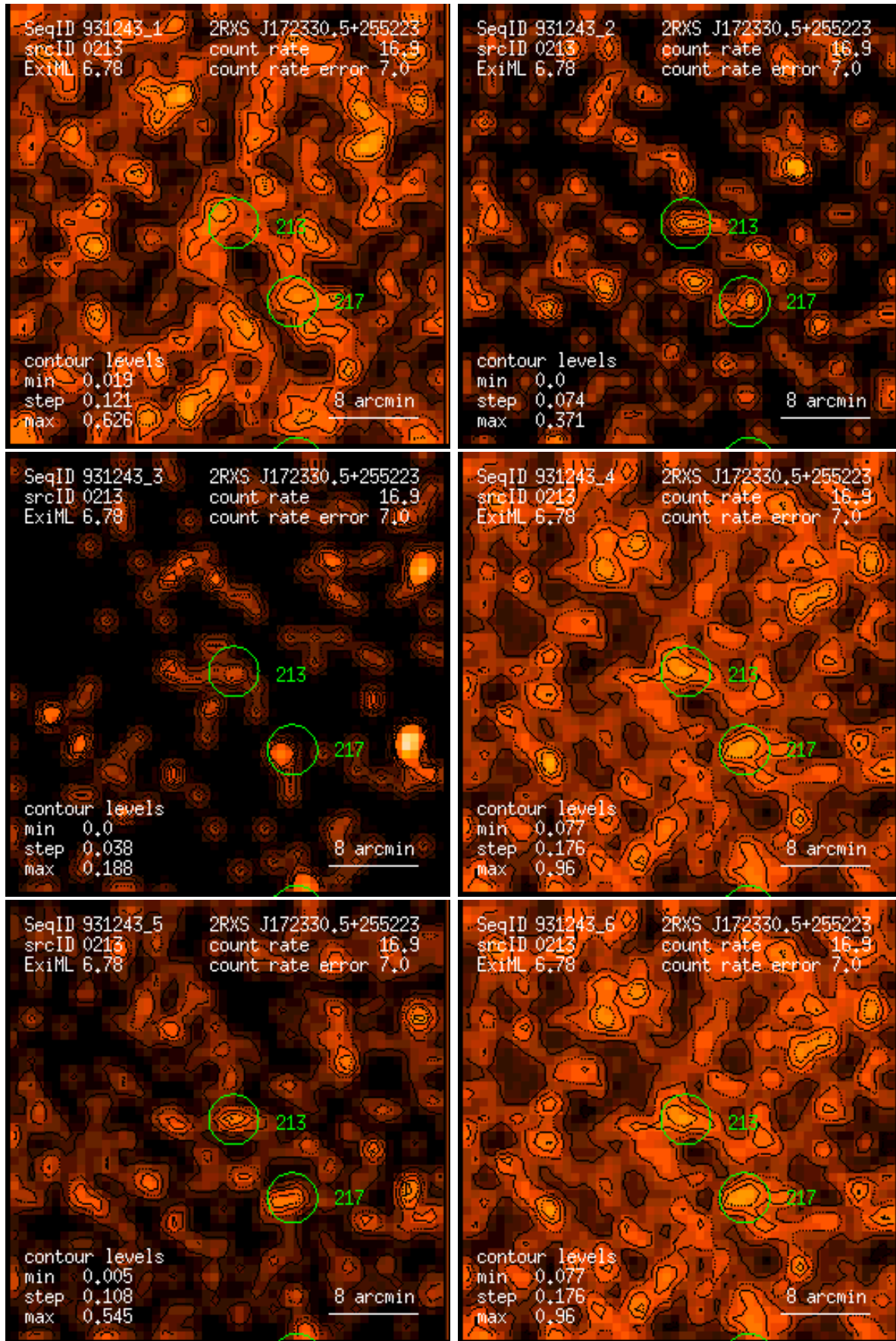
Figure 213: RASS 931243: detection 0213: band rate images, Gaussian filter: (1) PSPC channels 11 – 41, (2) 52 – 90, (3) 91 – 201, (4) 11 – 235, (5) 52 – 201, (6) 11 – 201. Broad band rates in counts/ks. Band rate contour levels in counts/ks/arcmin 2 .
