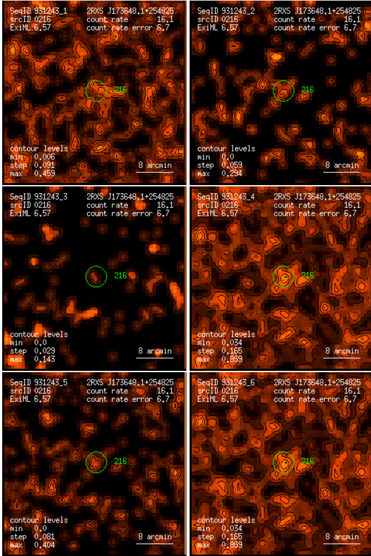
Figure 216: RASS 931243: detection 0216: band rate images, Gaussian filter: (1) PSPC channels 11 – 41, (2) 52 – 90, (3) 91 – 201, (4) 11 – 235, (5) 52 – 201, (6) 11 – 201. Broad band rates in counts/ks. Band rate contour levels in counts/ks/arcmin 2 .
