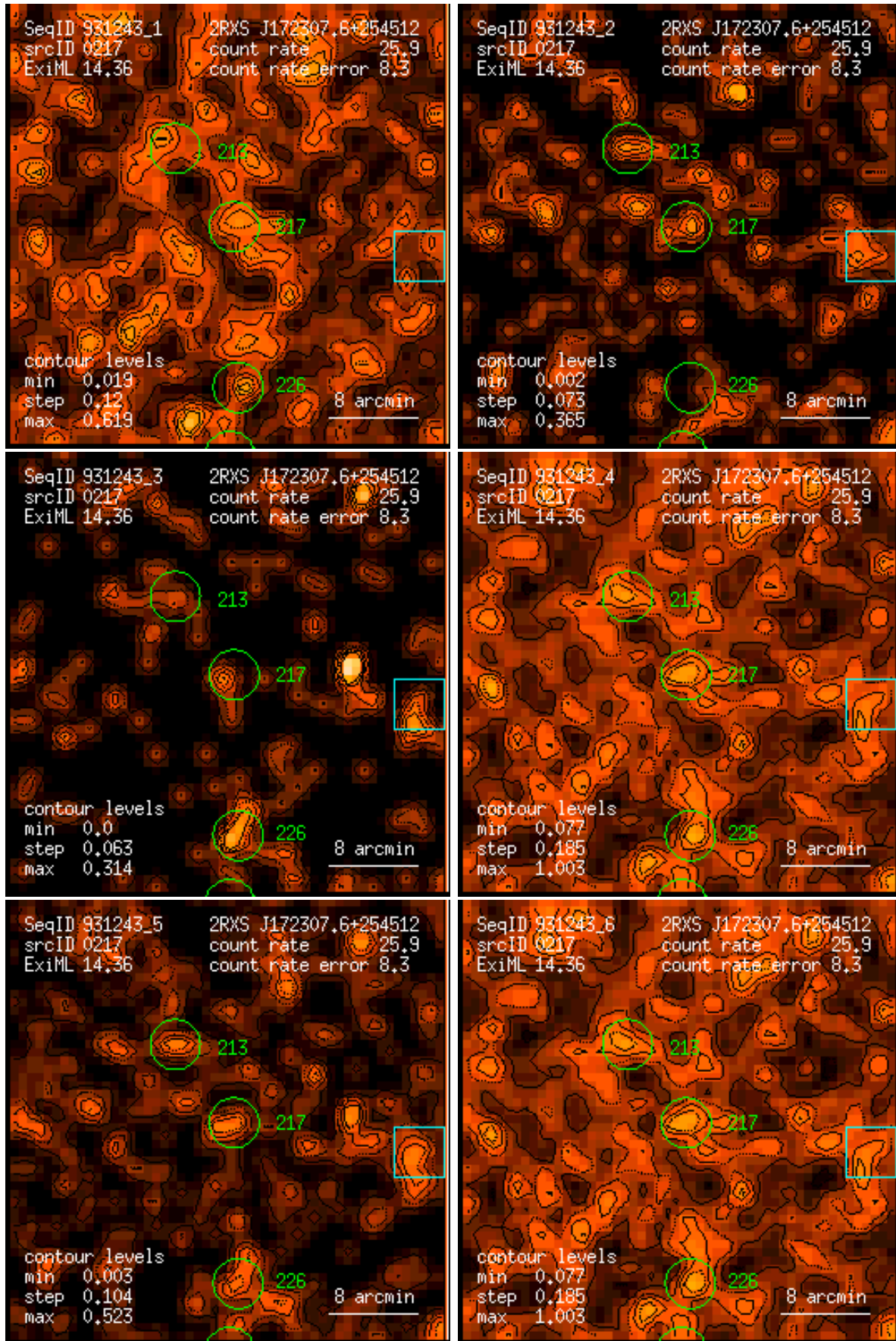
Figure 217: RASS 931243: detection 0217: band rate images, Gaussian filter: (1) PSPC channels 11 – 41, (2) 52 – 90, (3) 91 – 201, (4) 11 – 235, (5) 52 – 201, (6) 11 – 201. Broad band rates in counts/ks. Band rate contour levels in counts/ks/arcmin 2 .
