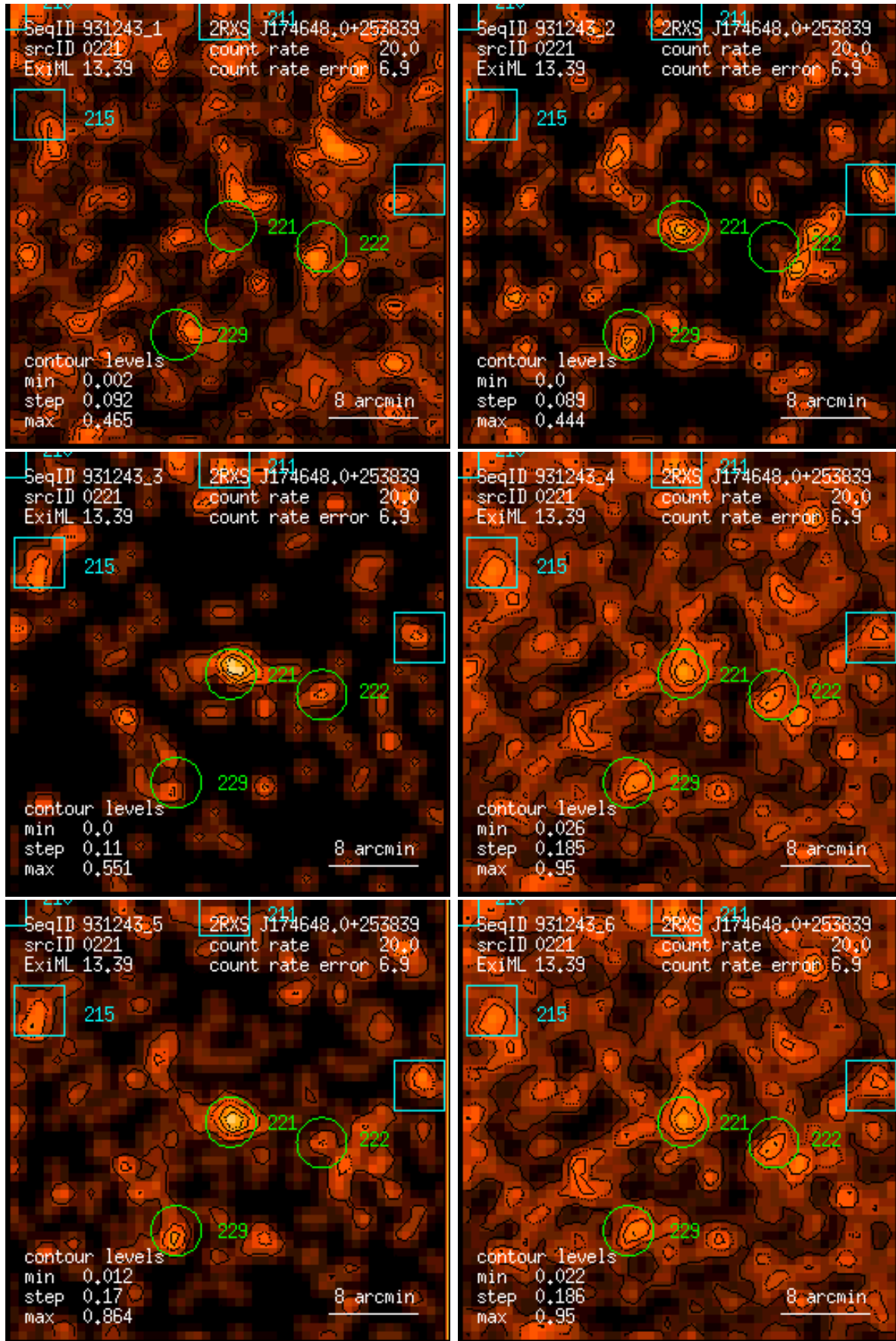
Figure 221: RASS 931243: detection 0221: band rate images, Gaussian filter: (1) PSPC channels 11 – 41, (2) 52 – 90, (3) 91 – 201, (4) 11 – 235, (5) 52 – 201, (6) 11 – 201. Broad band rates in counts/ks. Band rate contour levels in counts/ks/arcmin 2 .
