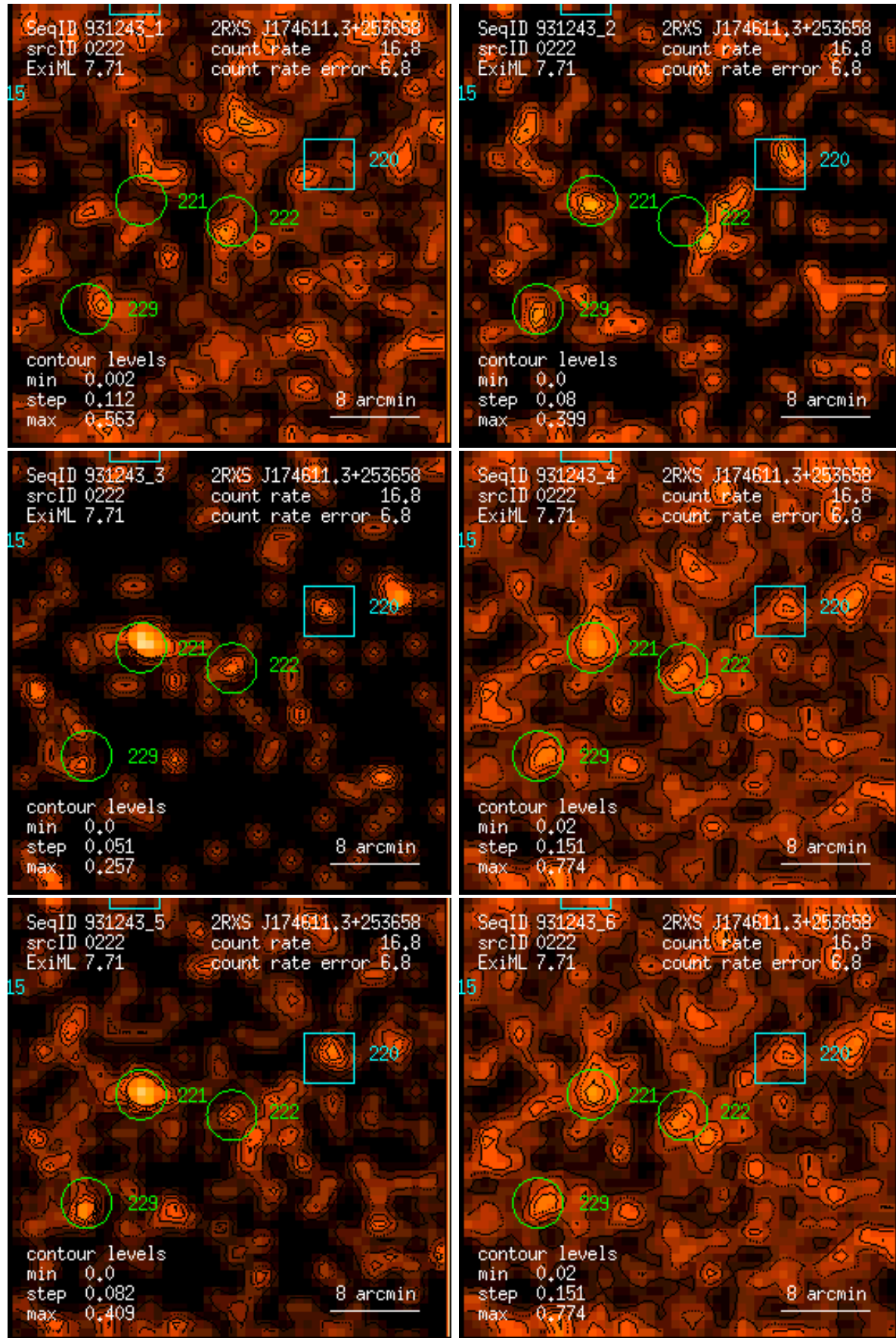
Figure 222: RASS 931243: detection 0222: band rate images, Gaussian filter: (1) PSPC channels 11 – 41, (2) 52 – 90, (3) 91 – 201, (4) 11 – 235, (5) 52 – 201, (6) 11 – 201. Broad band rates in counts/ks. Band rate contour levels in counts/ks/arcmin 2 .
