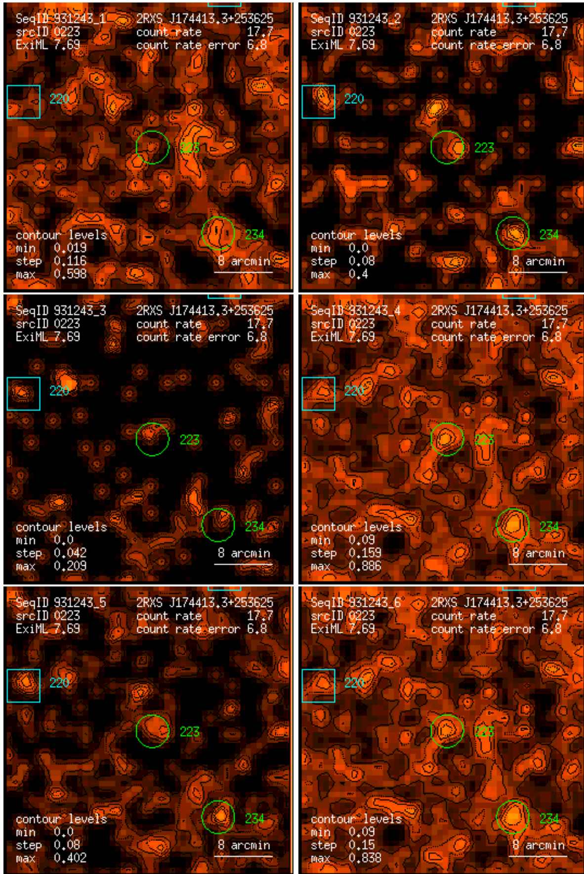
Figure 223: RASS 931243: detection 0223: band rate images, Gaussian filter: (1) PSPC channels 11 – 41, (2) 52 – 90, (3) 91 – 201, (4) 11 – 235, (5) 52 – 201, (6) 11 – 201. Broad band rates in counts/ks. Band rate contour levels in counts/ks/arcmin 2 .
