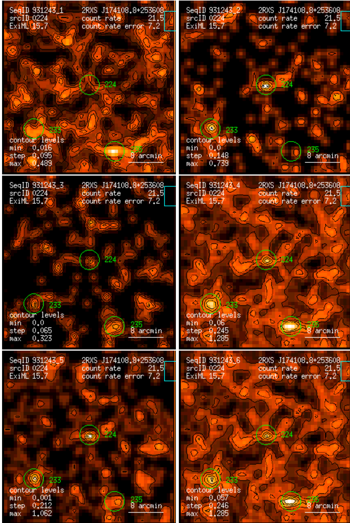
Figure 224: RASS 931243: detection 0224: band rate images, Gaussian filter: (1) PSPC channels 11 – 41, (2) 52 – 90, (3) 91 – 201, (4) 11 – 235, (5) 52 – 201, (6) 11 – 201. Broad band rates in counts/ks. Band rate contour levels in counts/ks/arcmin 2 .
