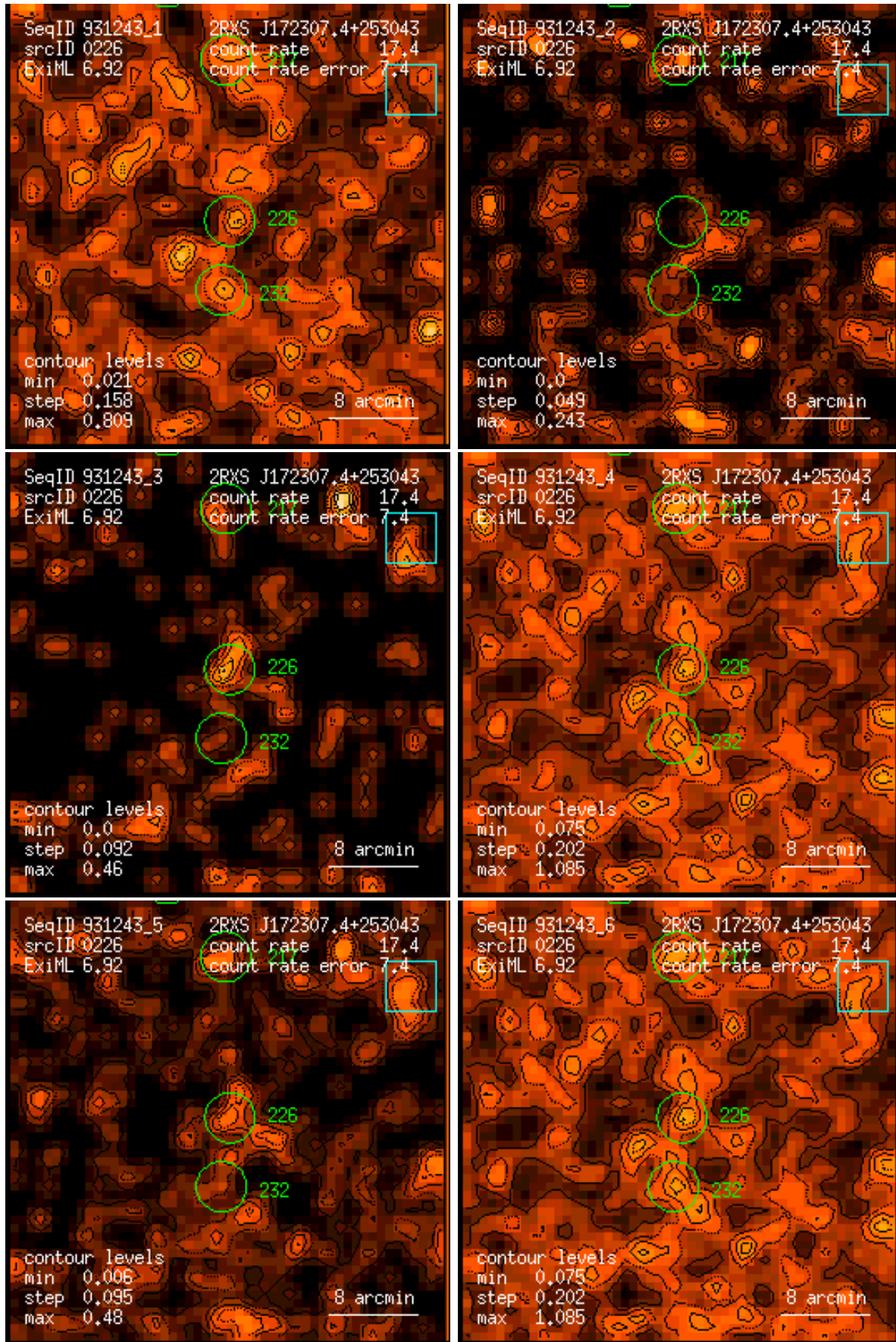
Figure 226: RASS 931243: detection 0226: band rate images, Gaussian filter: (1) PSPC channels 11 – 41, (2) 52 – 90, (3) 91 – 201, (4) 11 – 235, (5) 52 – 201, (6) 11 – 201. Broad band rates in counts/ks. Band rate contour levels in counts/ks/arcmin 2 .
