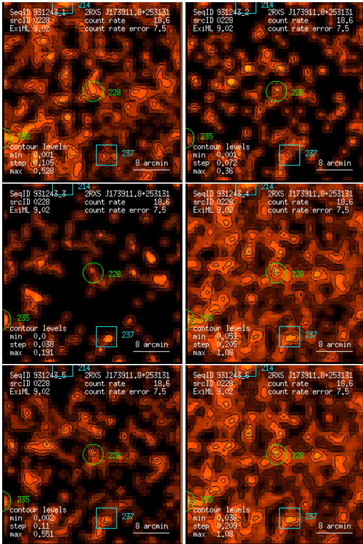
Figure 228: RASS 931243: detection 0228: band rate images, Gaussian filter: (1) PSPC channels 11 – 41, (2) 52 – 90, (3) 91 – 201, (4) 11 – 235, (5) 52 – 201, (6) 11 – 201. Broad band rates in counts/ks. Band rate contour levels in counts/ks/arcmin 2 .
