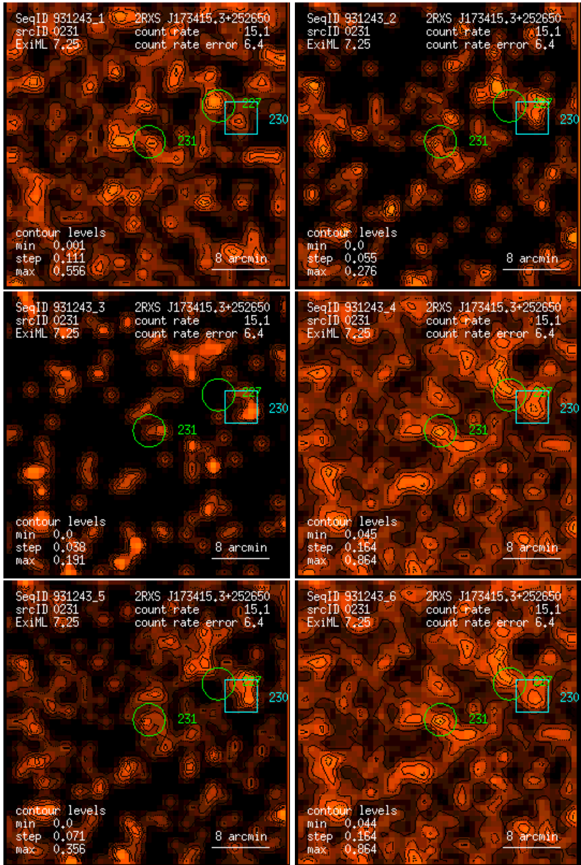
Figure 231: RASS 931243: detection 0231: band rate images, Gaussian filter: (1) PSPC channels 11 – 41, (2) 52 – 90, (3) 91 – 201, (4) 11 – 235, (5) 52 – 201, (6) 11 – 201. Broad band rates in counts/ks. Band rate contour levels in counts/ks/arcmin 2 .
