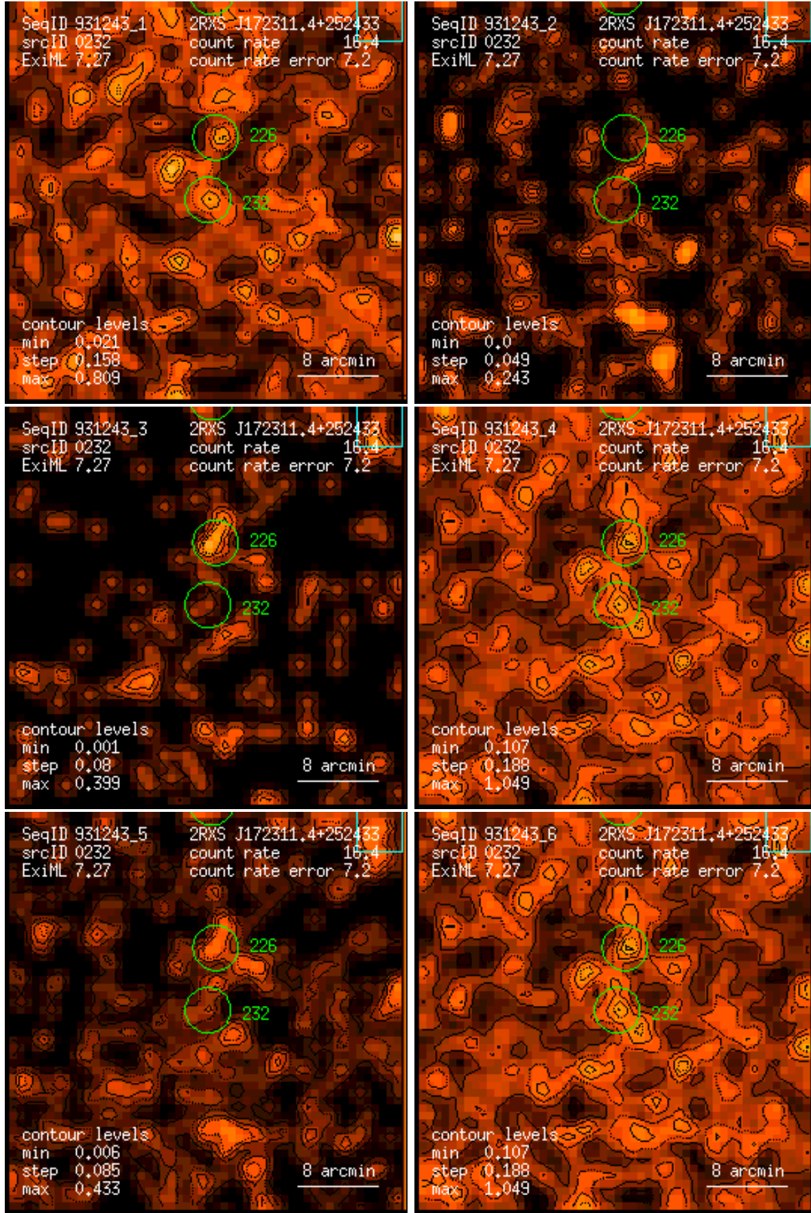
Figure 232: RASS 931243: detection 0232: band rate images, Gaussian filter: (1) PSPC channels 11 – 41, (2) 52 – 90, (3) 91 – 201, (4) 11 – 235, (5) 52 – 201, (6) 11 – 201. Broad band rates in counts/ks. Band rate contour levels in counts/ks/arcmin 2 .
