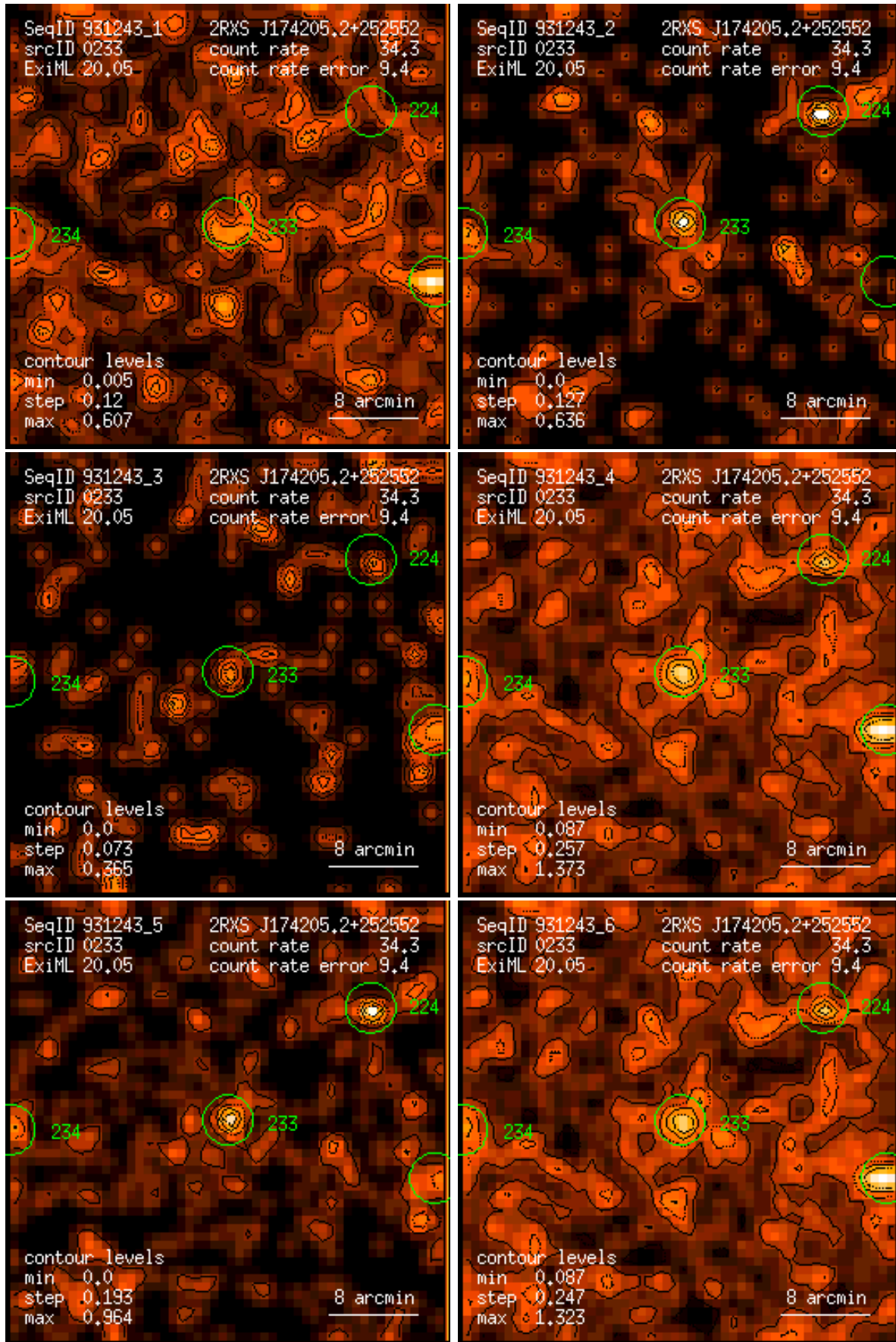
Figure 233: RASS 931243: detection 0233: band rate images, Gaussian filter: (1) PSPC channels 11 – 41, (2) 52 – 90, (3) 91 – 201, (4) 11 – 235, (5) 52 – 201, (6) 11 – 201. Broad band rates in counts/ks. Band rate contour levels in counts/ks/arcmin 2 .
