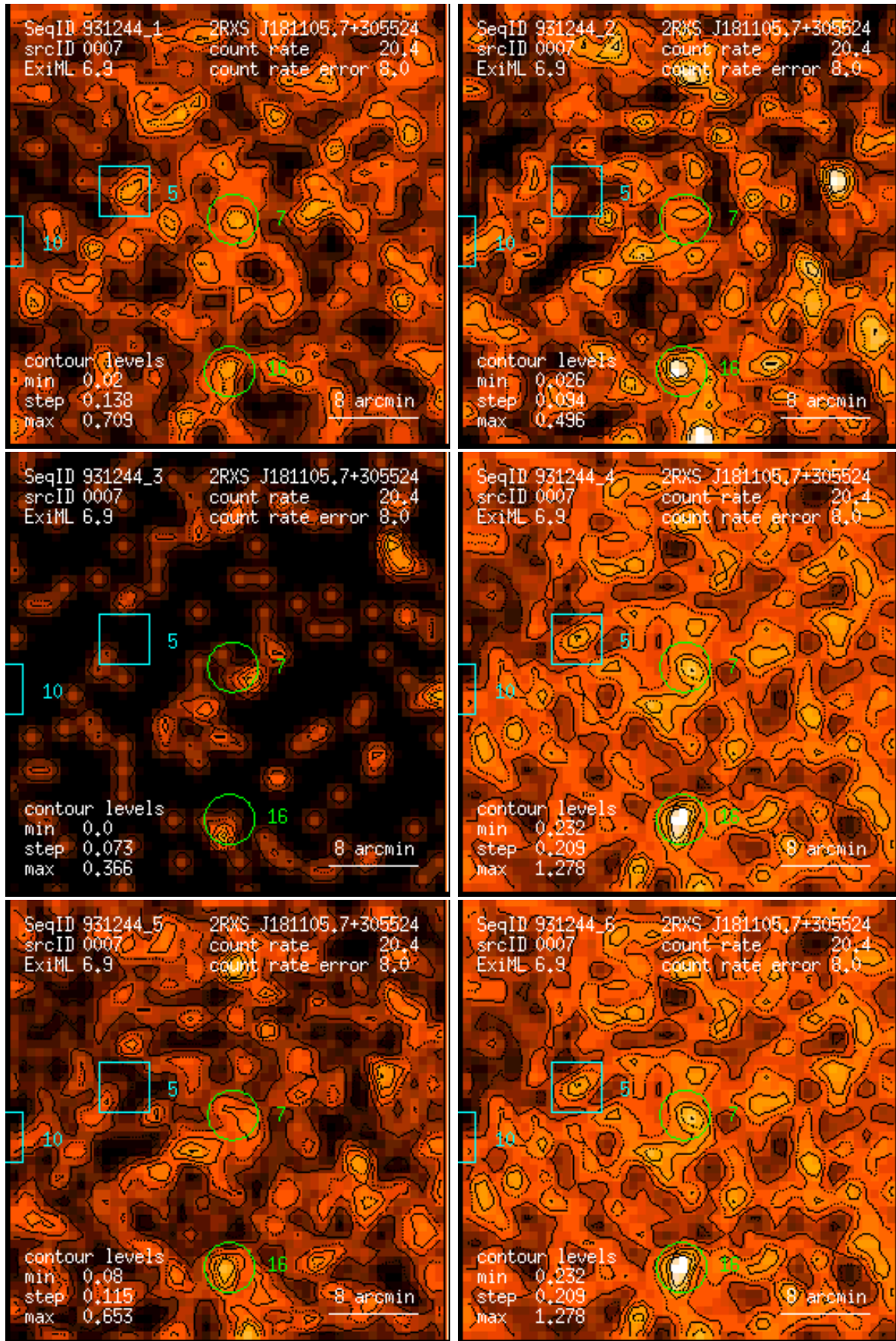
Figure 7: RASS 931244: detection 0007: band rate images, Gaussian filter: (1) PSPC channels 11 – 41, (2) 52 – 90, (3) 91 – 201, (4) 11 – 235, (5) 52 – 201, (6) 11 – 201. Broad band rates in counts/ks. Band rate contour levels in counts/ks/arcmin 2 .
