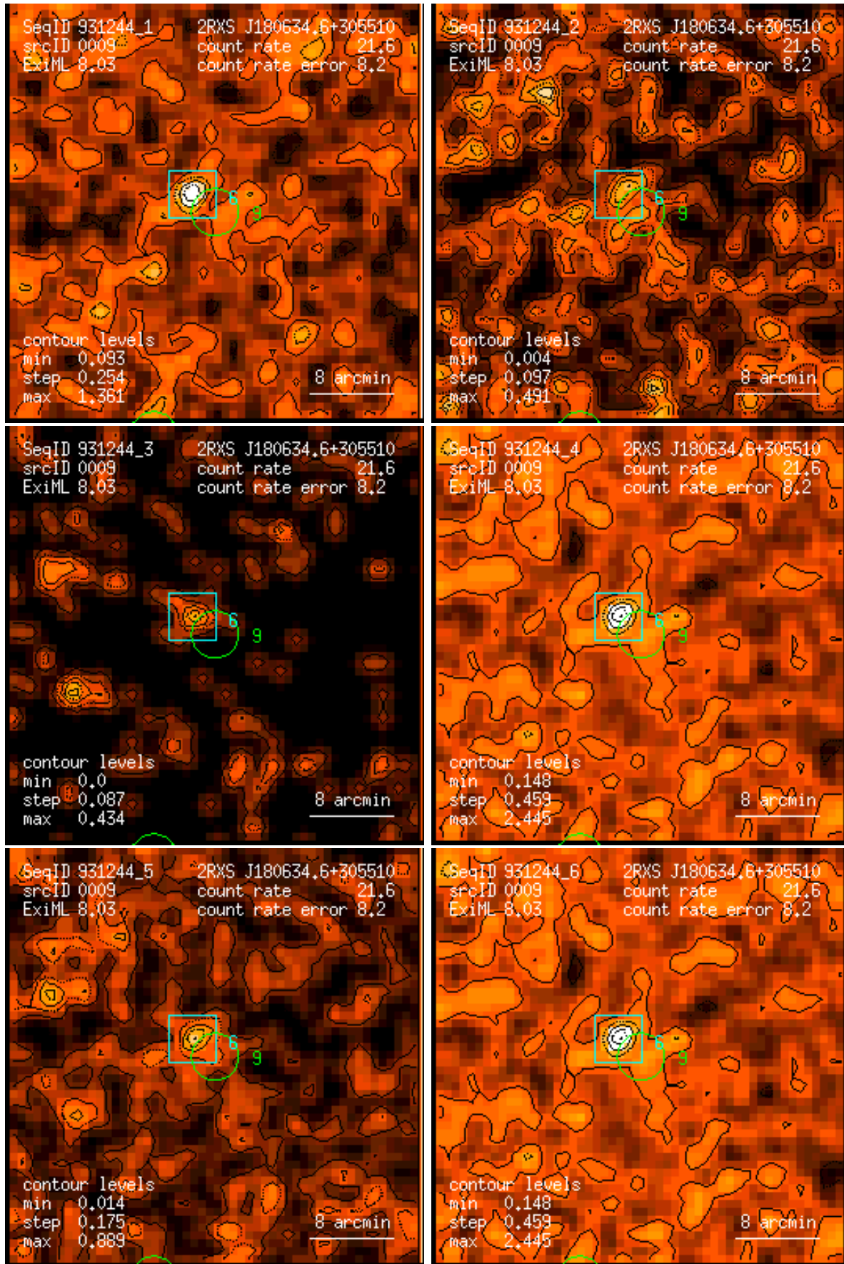
Figure 9: RASS 931244: detection 0009: band rate images, Gaussian filter: (1) PSPC channels 11 – 41, (2) 52 – 90, (3) 91 – 201, (4) 11 – 235, (5) 52 – 201, (6) 11 – 201. Broad band rates in counts/ks. Band rate contour levels in counts/ks/arcmin 2 .
