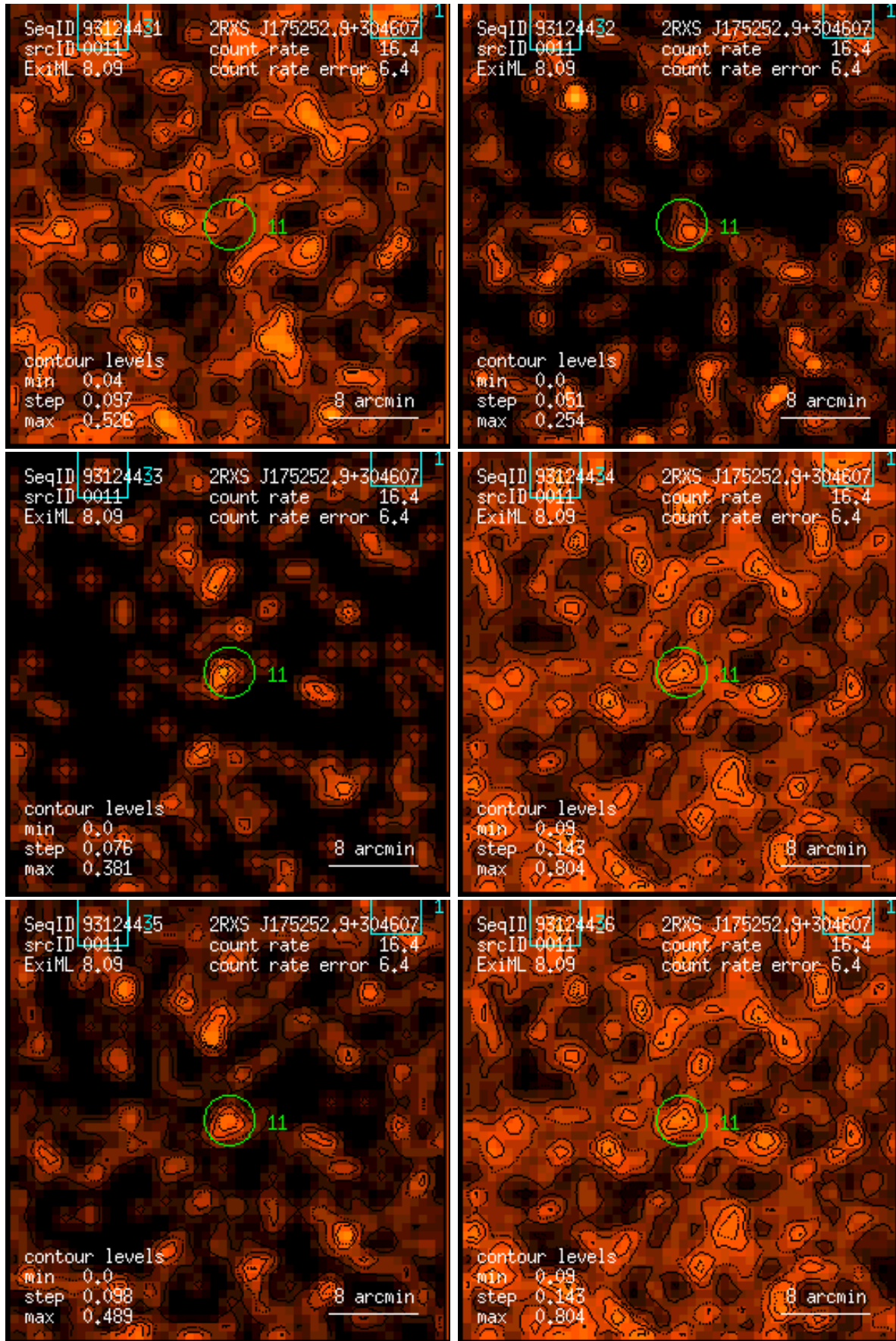
Figure 11: RASS 931244: detection 0011: band rate images, Gaussian filter: (1) PSPC channels 11 – 41, (2) 52 – 90, (3) 91 – 201, (4) 11 – 235, (5) 52 – 201, (6) 11 – 201. Broad band rates in counts/ks. Band rate contour levels in counts/ks/arcmin 2 .
