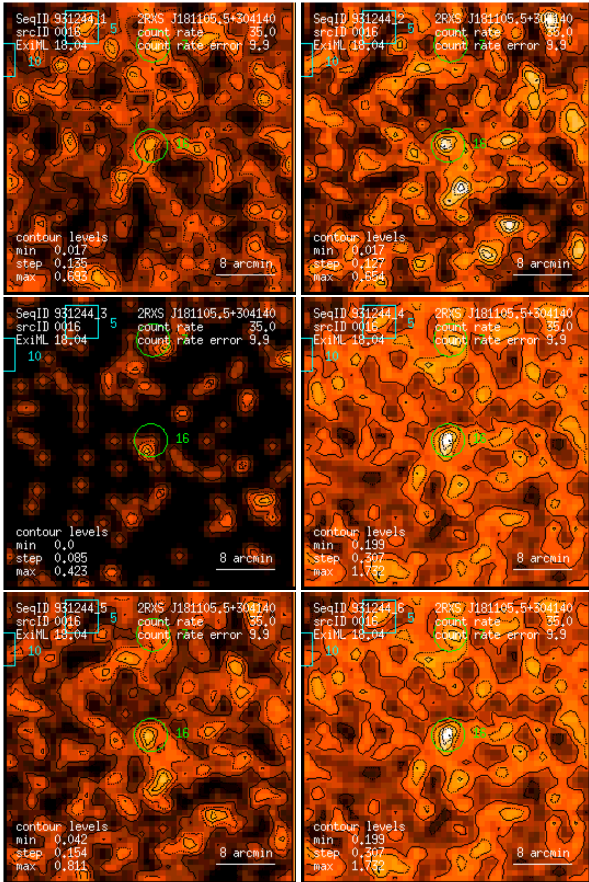
Figure 16: RASS 931244: detection 0016: band rate images, Gaussian filter: (1) PSPC channels 11 – 41, (2) 52 – 90, (3) 91 – 201, (4) 11 – 235, (5) 52 – 201, (6) 11 – 201. Broad band rates in counts/ks. Band rate contour levels in counts/ks/arcmin 2 .
