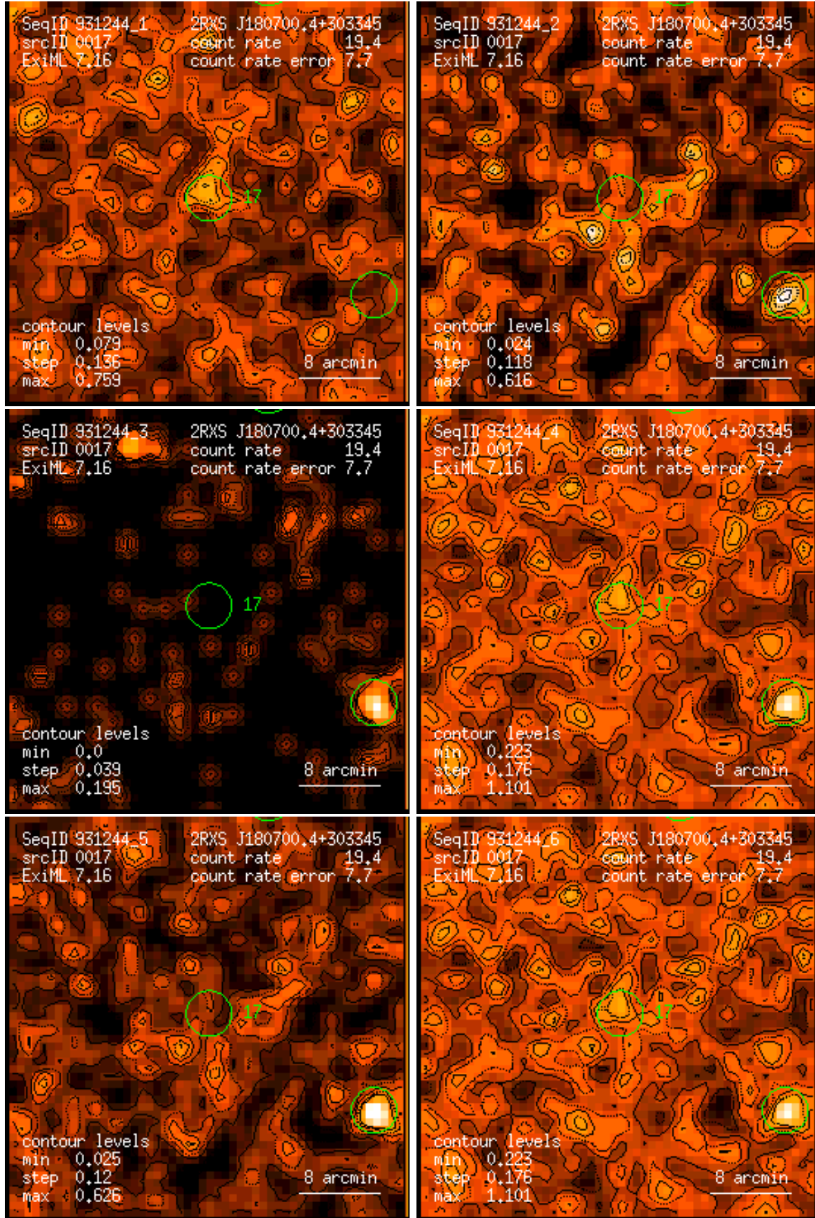
Figure 17: RASS 931244: detection 0017: band rate images, Gaussian filter: (1) PSPC channels 11 – 41, (2) 52 – 90, (3) 91 – 201, (4) 11 – 235, (5) 52 – 201, (6) 11 – 201. Broad band rates in counts/ks. Band rate contour levels in counts/ks/arcmin 2 .
