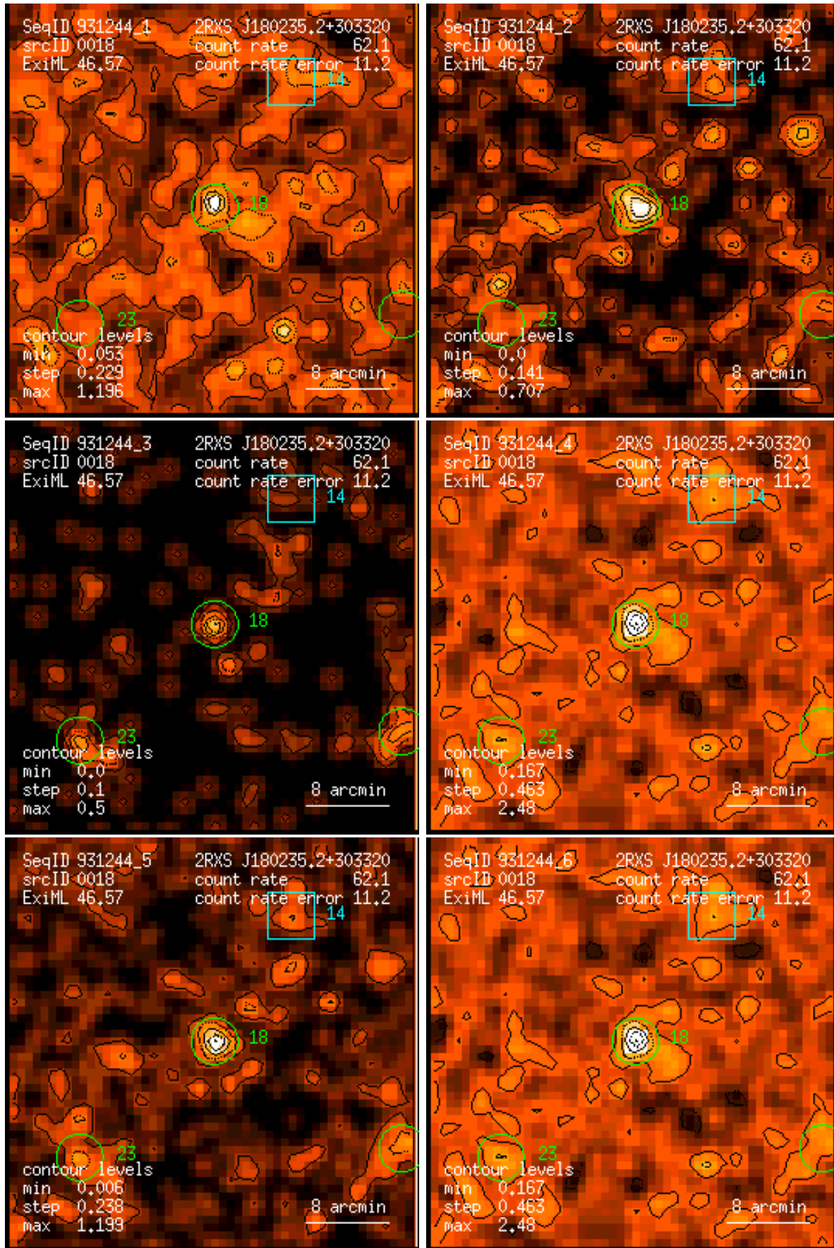
Figure 18: RASS 931244: detection 0018: band rate images, Gaussian filter: (1) PSPC channels 11 – 41, (2) 52 – 90, (3) 91 – 201, (4) 11 – 235, (5) 52 – 201, (6) 11 – 201. Broad band rates in counts/ks. Band rate contour levels in counts/ks/arcmin 2 .
